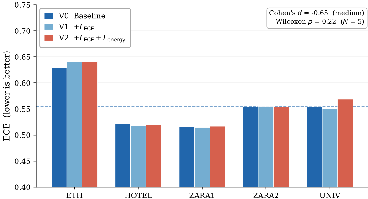
ECE across ETH-UCY folds: V0 baseline and loss ablations
