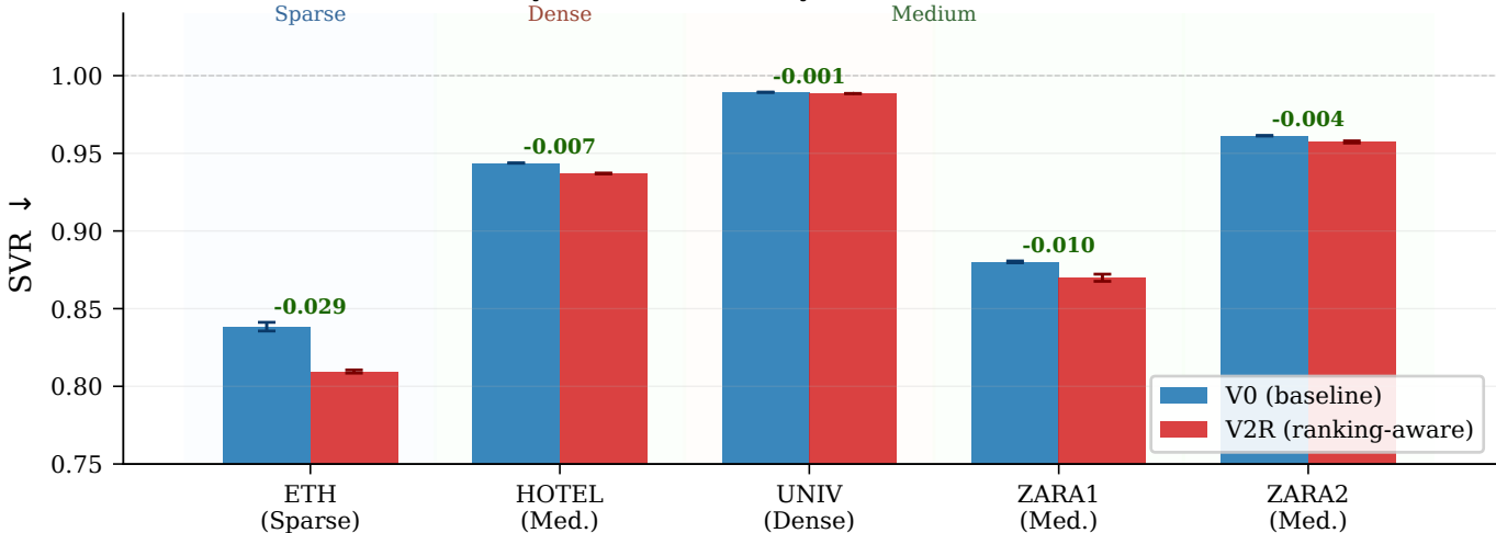
Social Violation Rate by Subset and Density Tier (3-seed mean \pm std; seeds 42, 1, 123)
