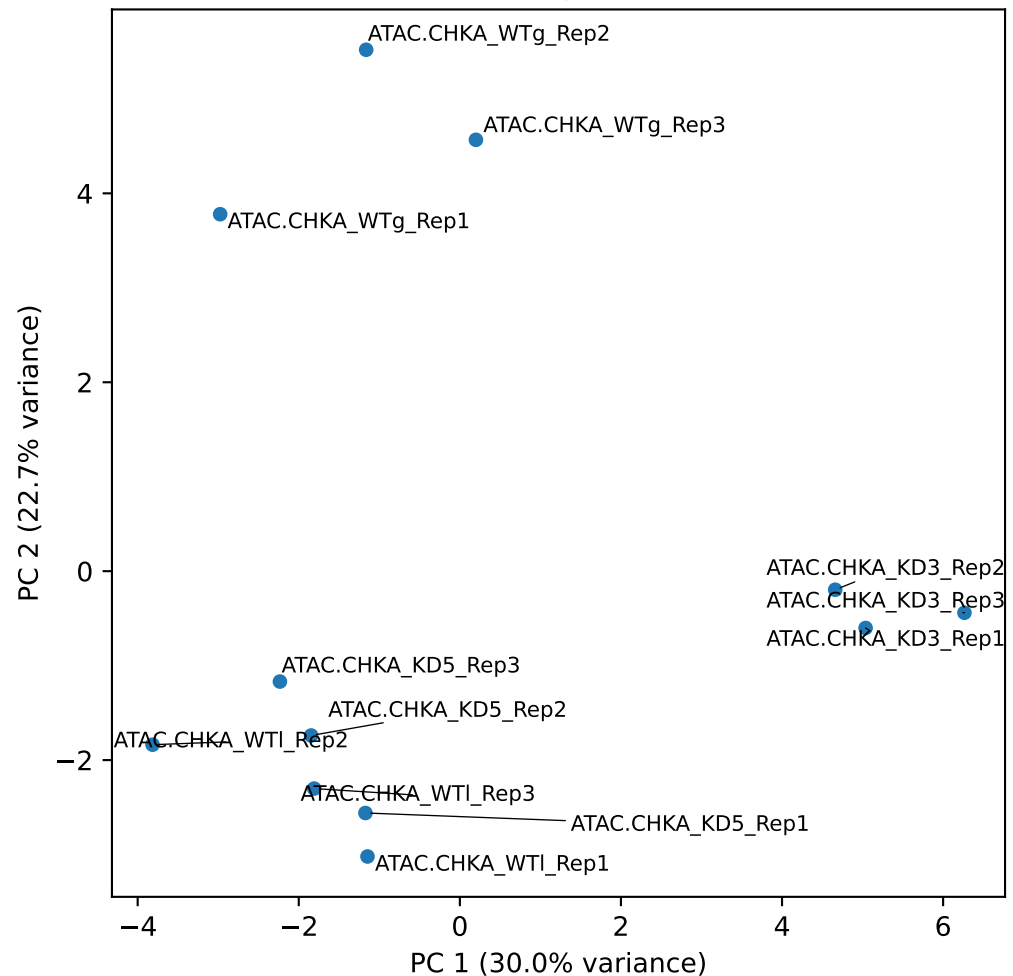
PCA based on Top 100 and bottom 100 regions (ordered by Log2FC); Cumulative number Data source:input.vout.anno
