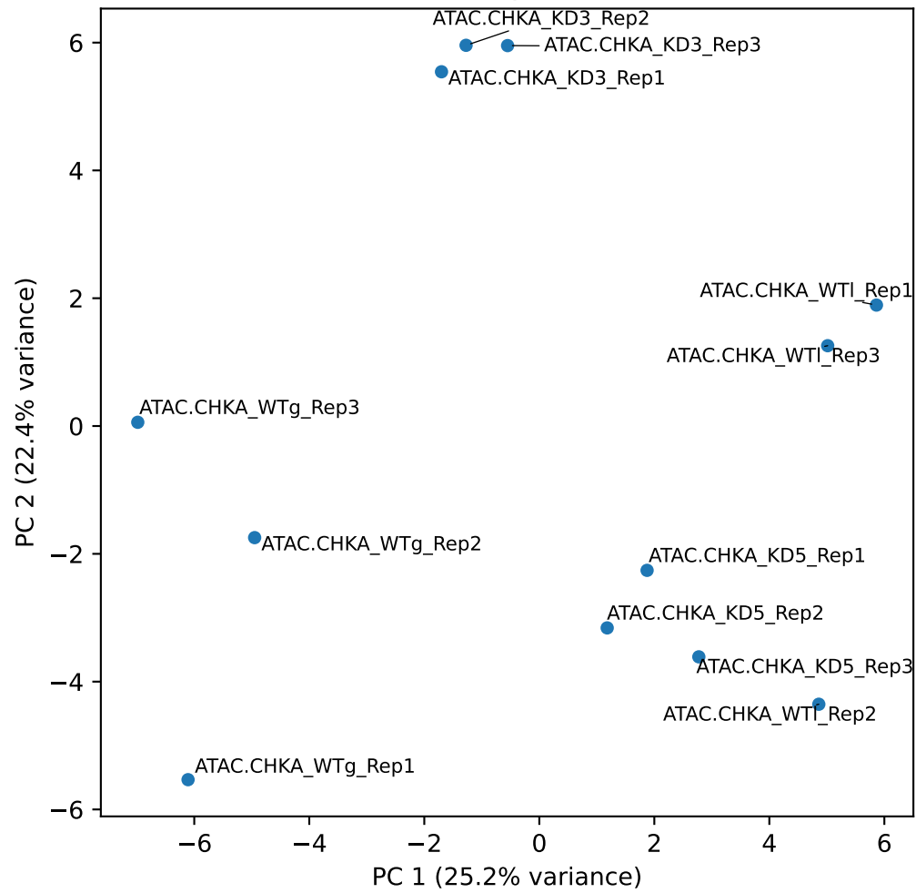
PCA based on 0 Up- and 627 Down-regulated regions (FDR<0.05); Cumulative number Data source:input.vout.anno
