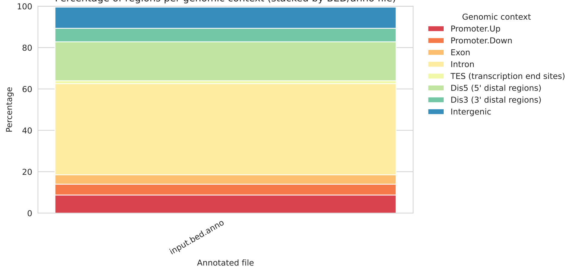
Percentage of regions per genomic context (stacked by BED/anno file)
