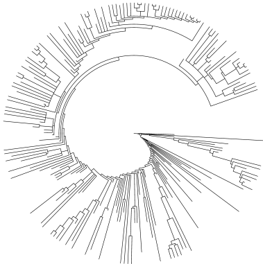
L2-Norm on 10 Princial Components
