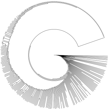
Cosine Distance
