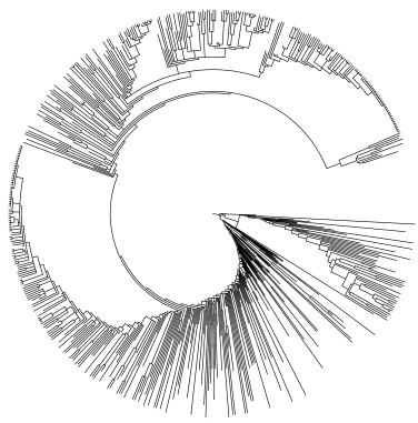
L2-Norm on 2 Princial Components
