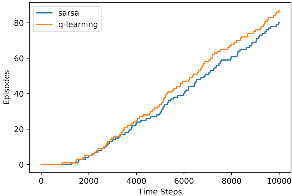
8-Direction King's Move Windy Grid World
