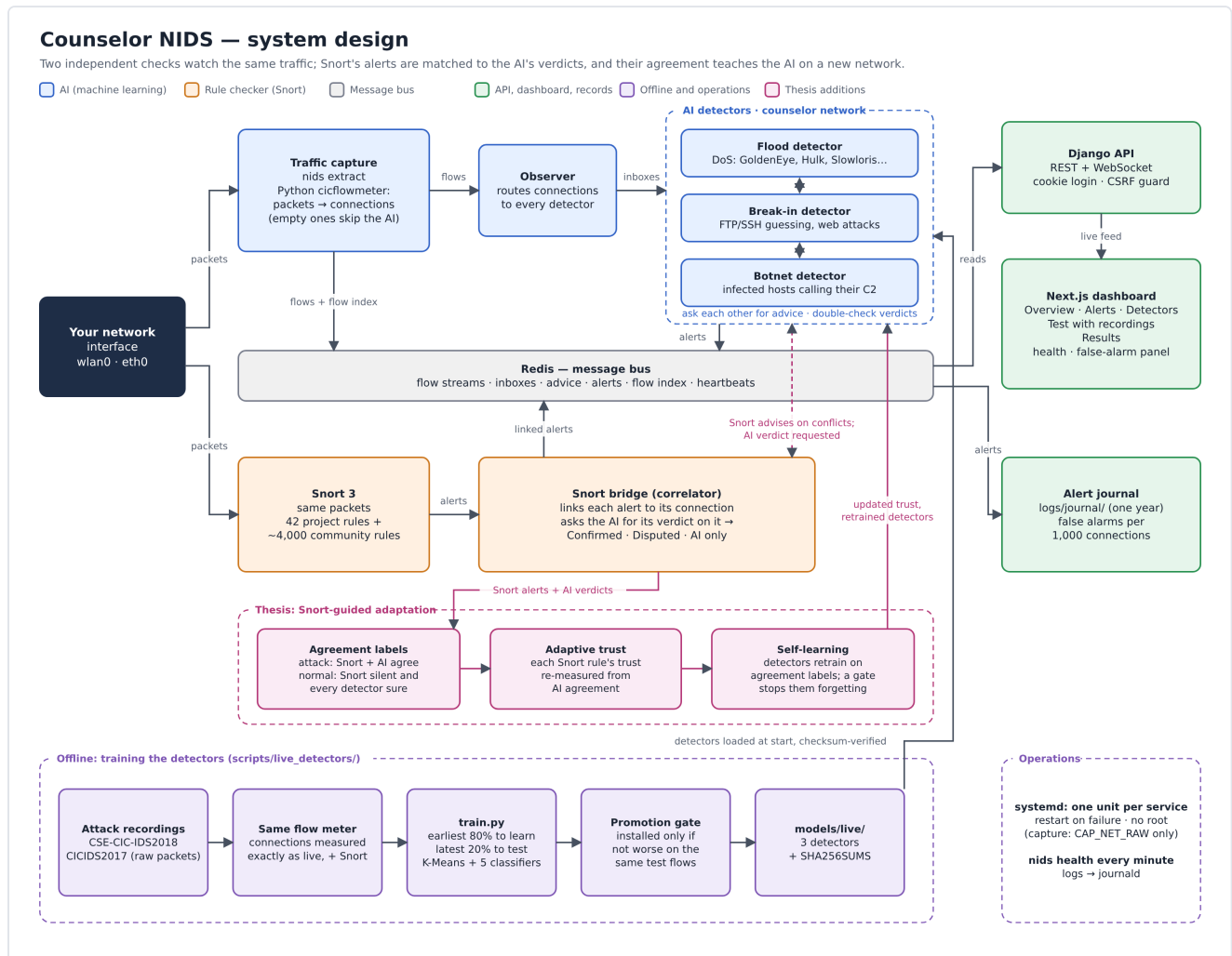
Figure 1. System design: two lanes judge the same packets; Redis carries the messages between services; the magenta row is the thesis addition.
