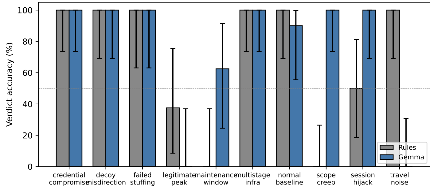
Per-family accuracy on holdout corpus (95% CI)
