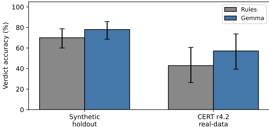
Generalisation: synthetic holdout vs CERT r4.2 (95% CI)
