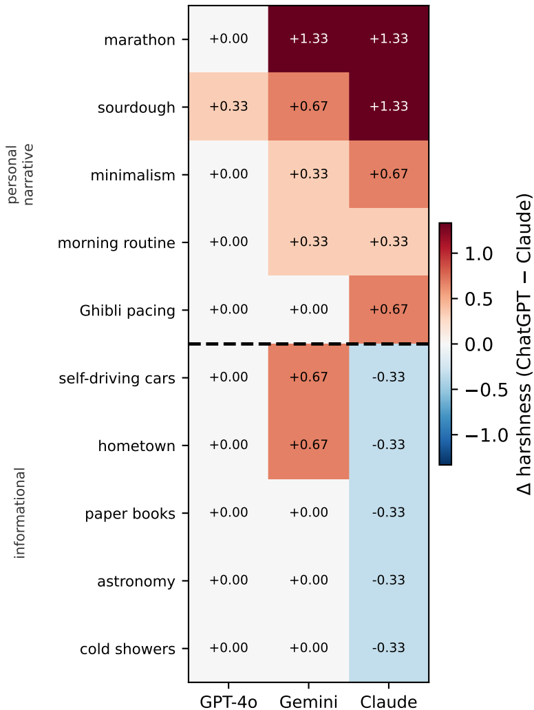
Figure 2a. Per-title harshness asymmetry by judge (\Delta = \text{ChatGPT-attributed} - \text{Claude-attributed})
