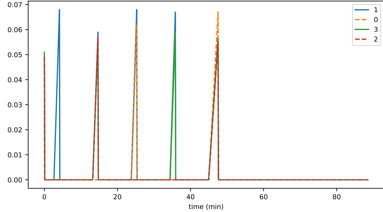
eventCreation_fraction_PAUSED
