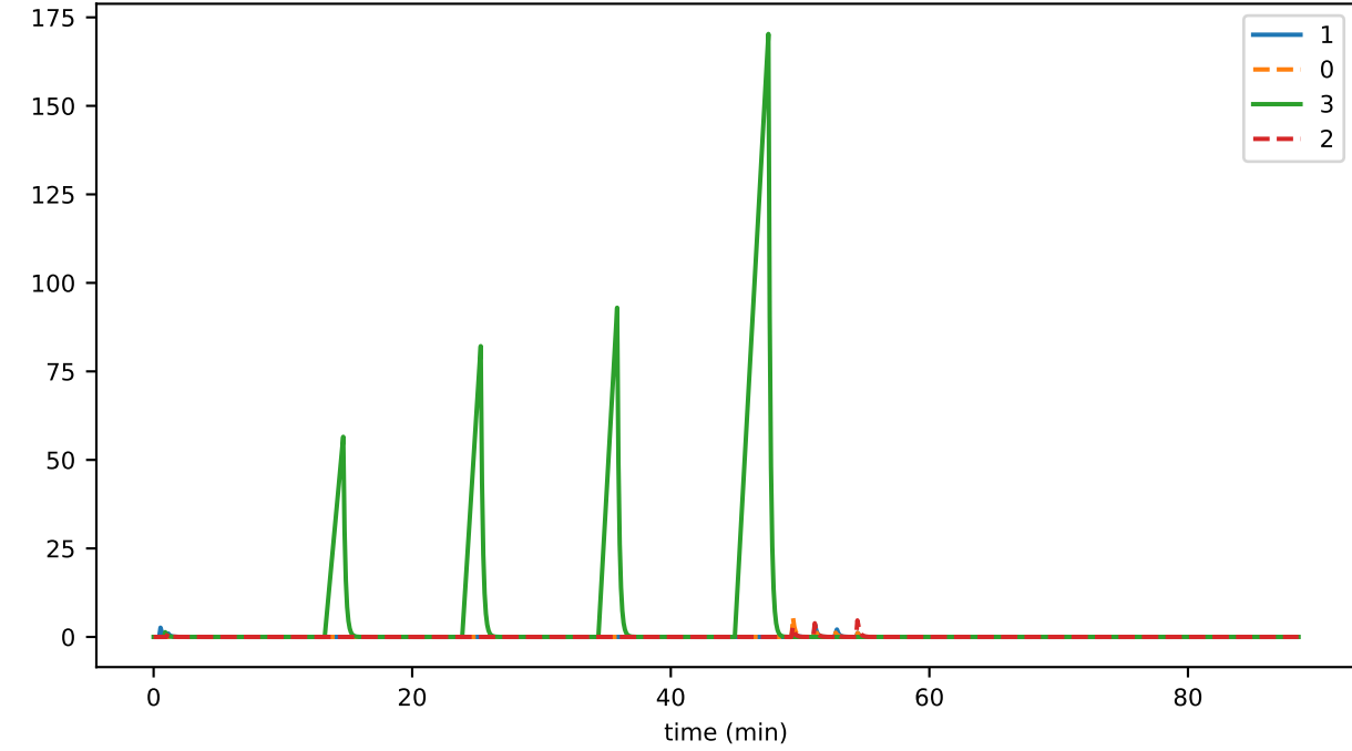
consEvents (q2)
