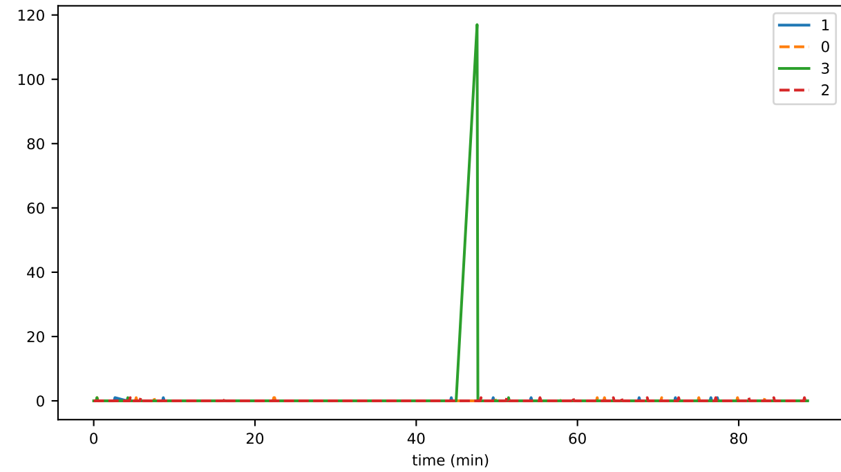
eventCreationManager_unhandled_task_count
