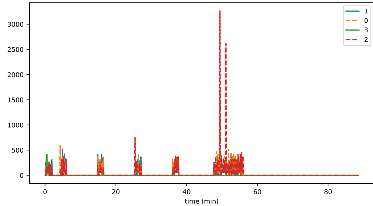
bytes/sec_sent
