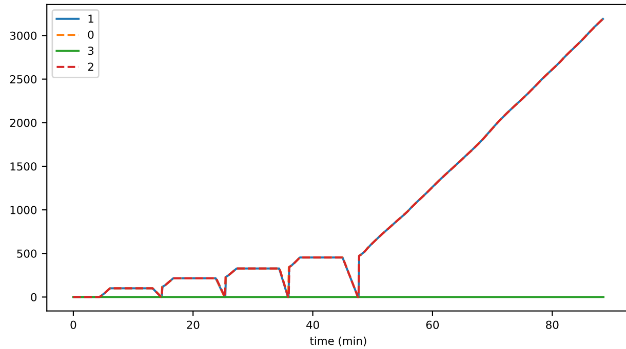
sec/sync1
