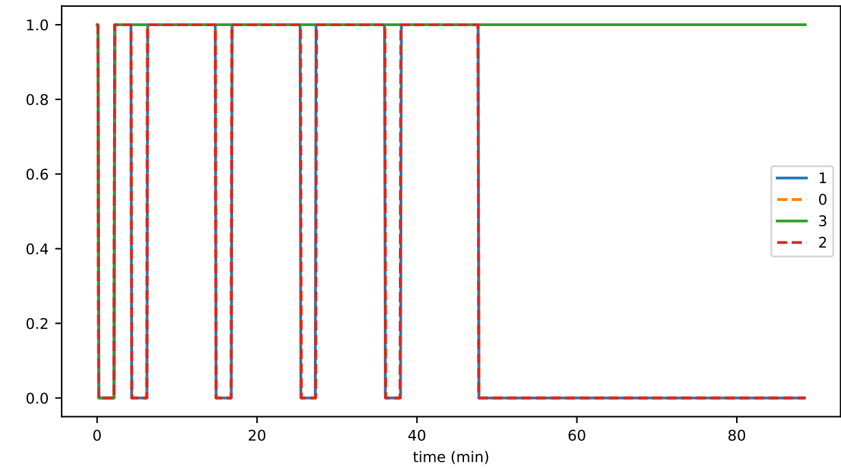
DigBatches/sec
