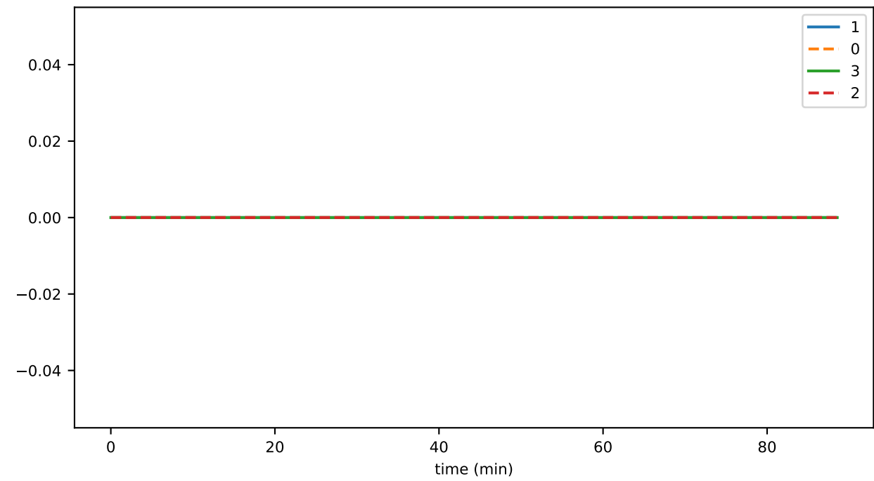
DigBatches/sec
