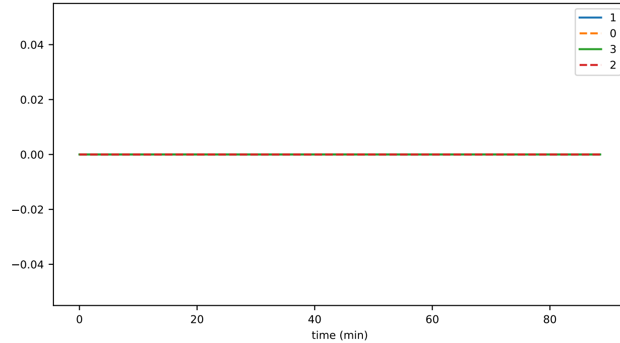
numOrphans
