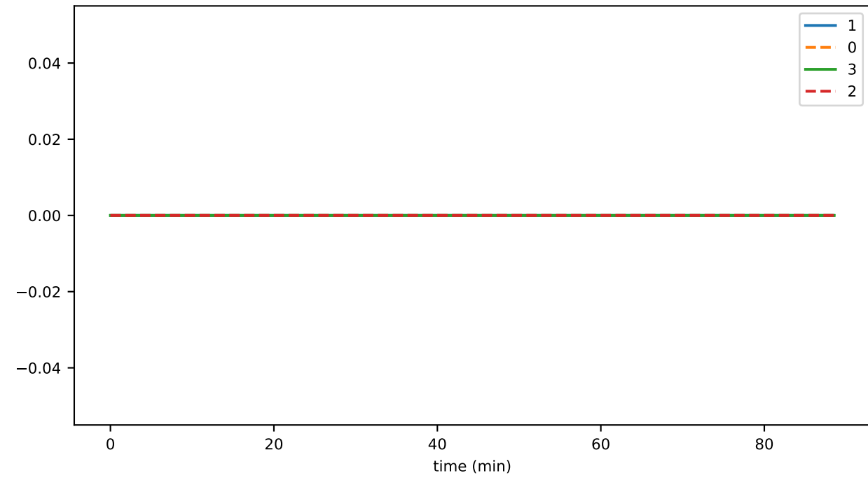
htFCMTimeMicroSec
