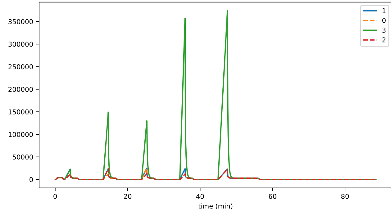
consEvents (q2)
