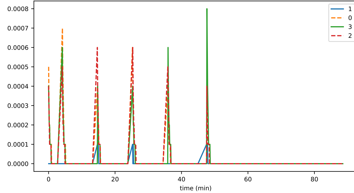
sec/sync2
