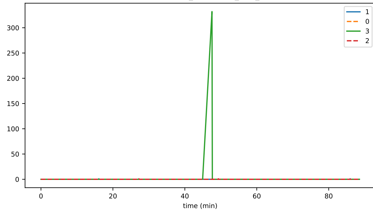
linkedEventIntake_unhandled_task_count
