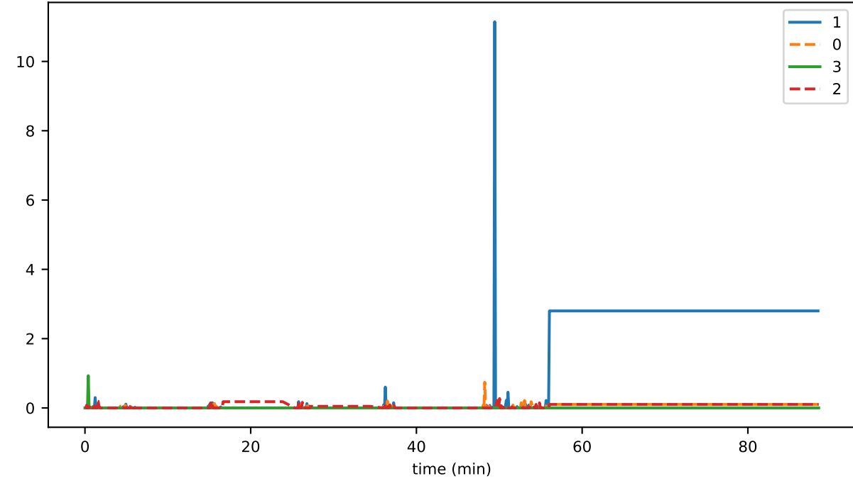
avgTransSubmitMicros
