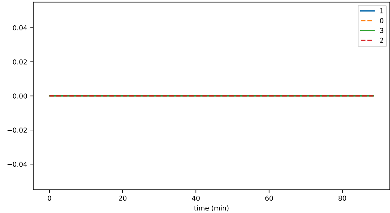
staleSystemTransactions
