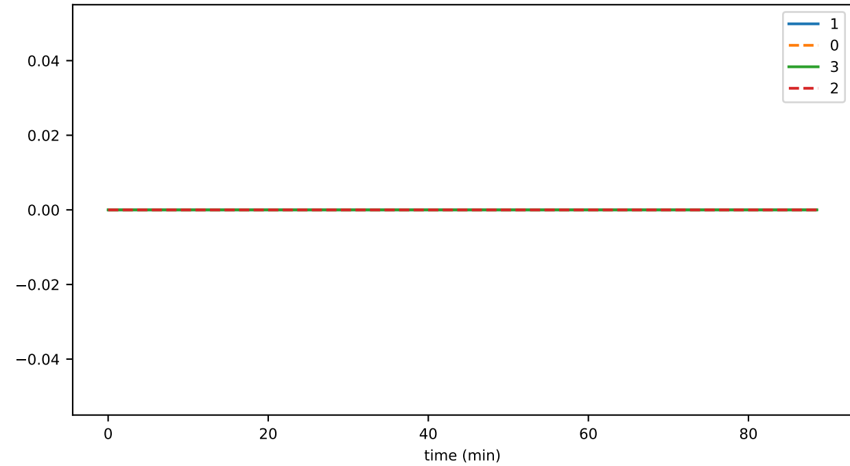
eventRecRate
