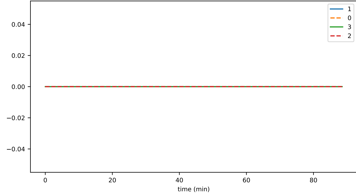
SigBatches/sec
