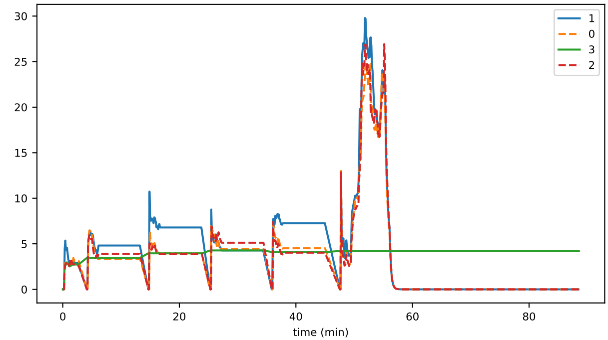
stateSignatureCollector_unhandled_task_count
