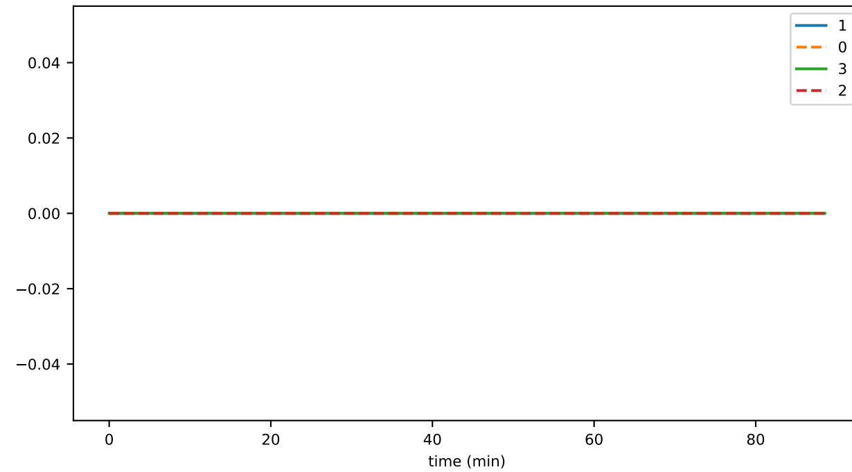
eventsWithNullHashedData
