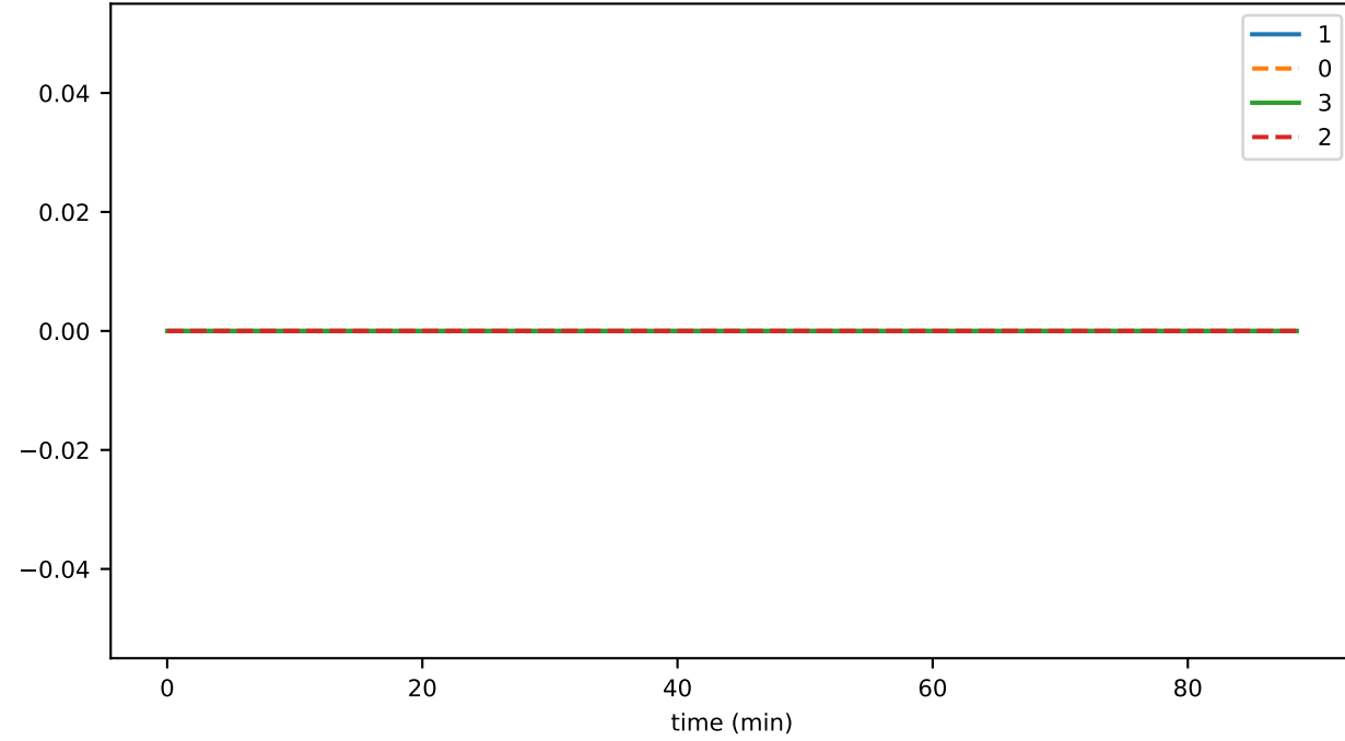
Sig/sec
