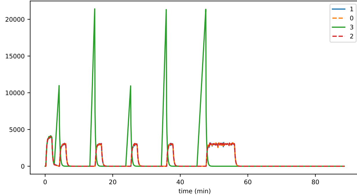
transH/sec
