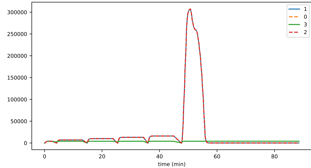
htFCQTimeMicroSec
