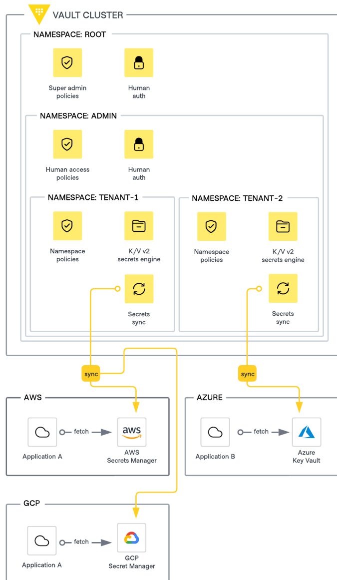
Figure 17: Secrets sync namespace design
