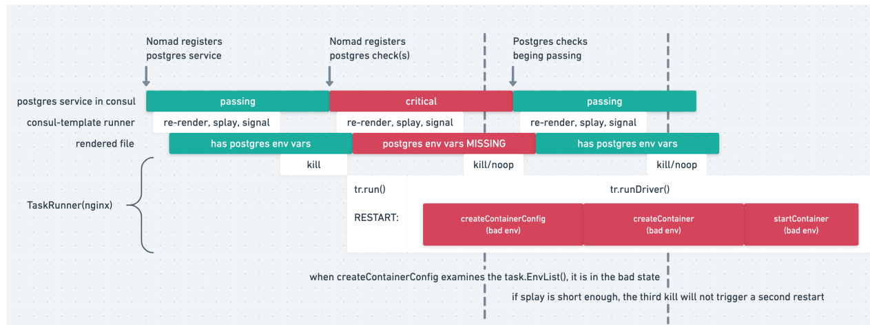
Figure 6: Template rendering flow
