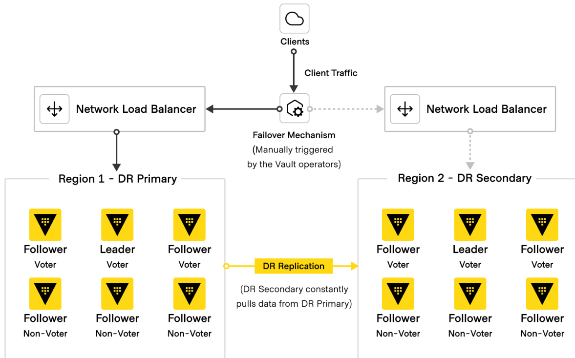
Figure 4: HVD Vault Disaster Recovery Diagram
