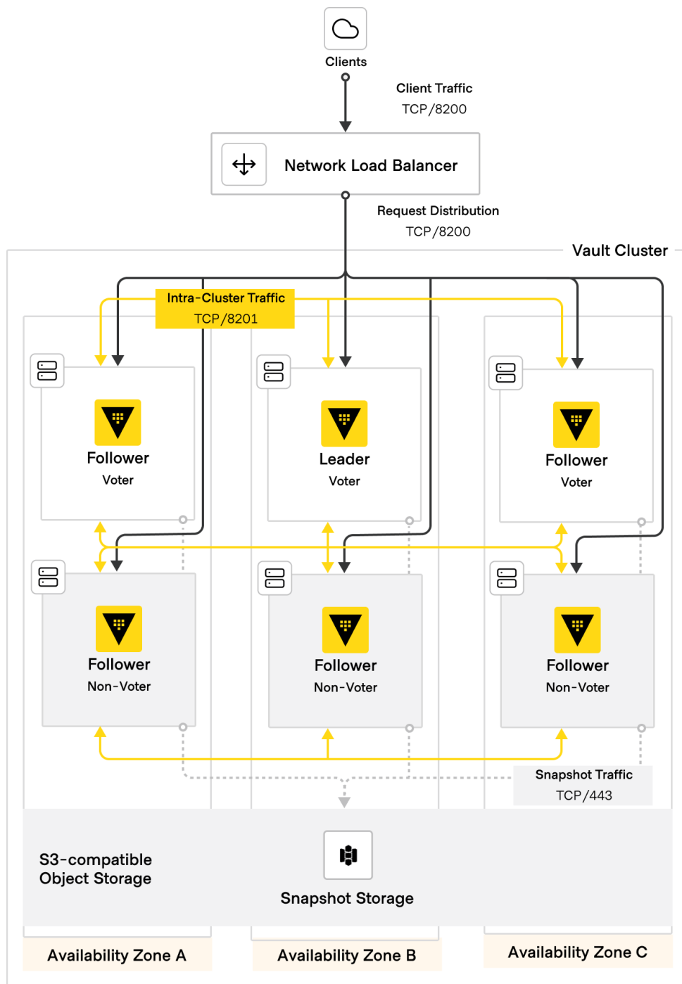
Figure 5: HVD Vault networking diagram
