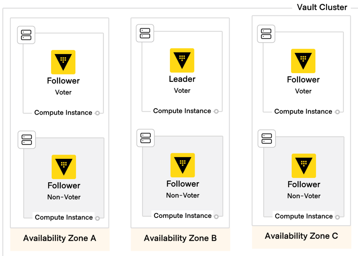
Figure 2: HVD Vault HA 6 nodes redundancy zones diagram
