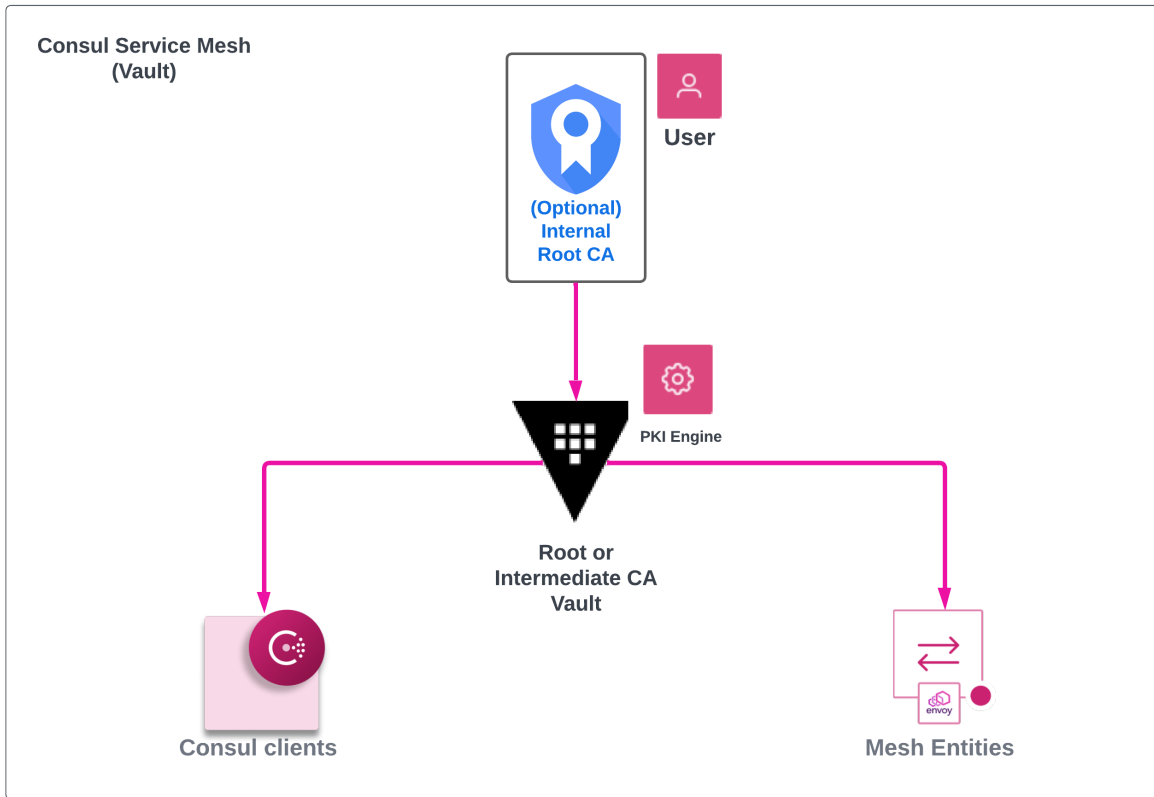
Figure 15: Vault as Consul CA
