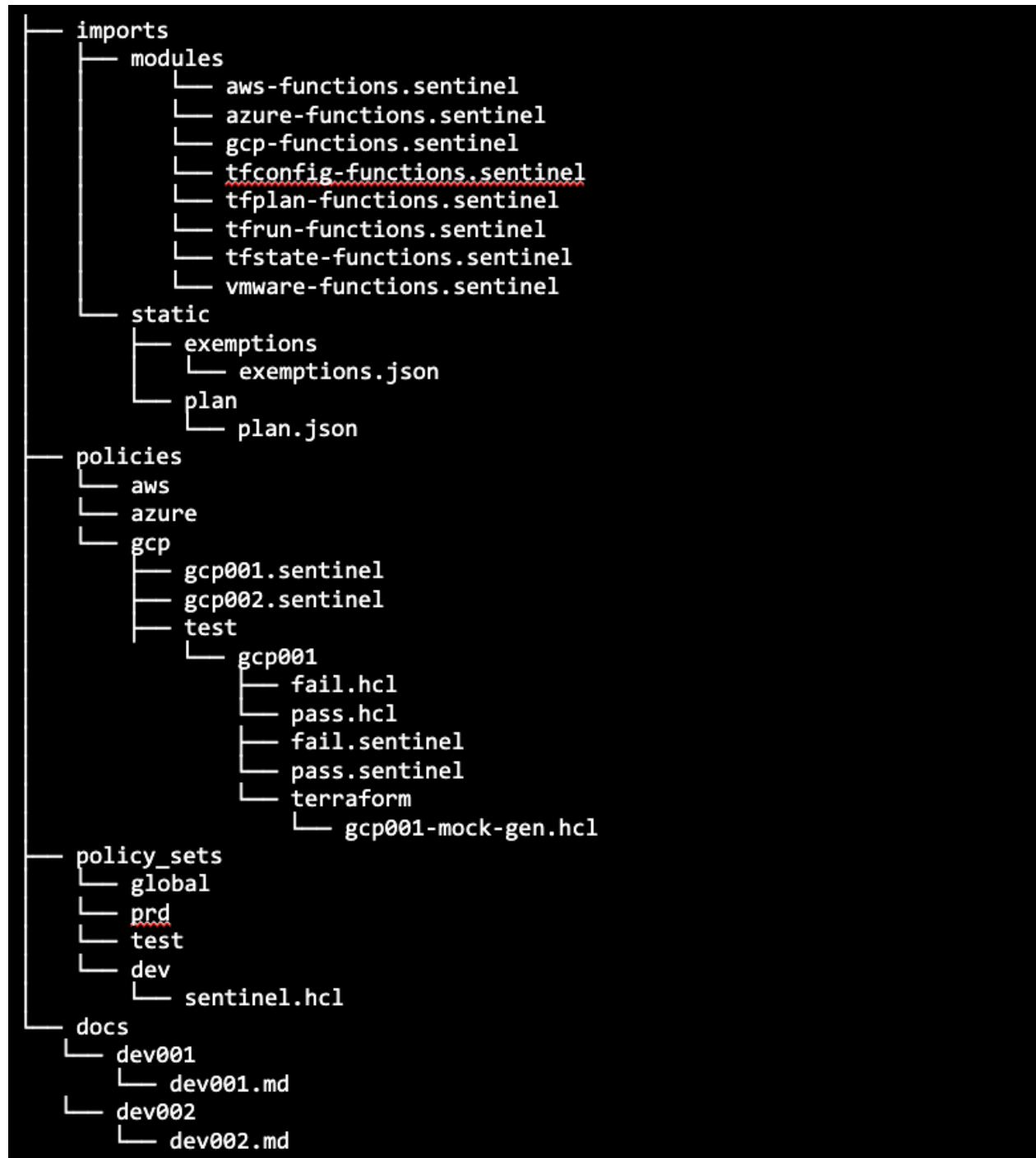
Figure 30: Repository Organization
