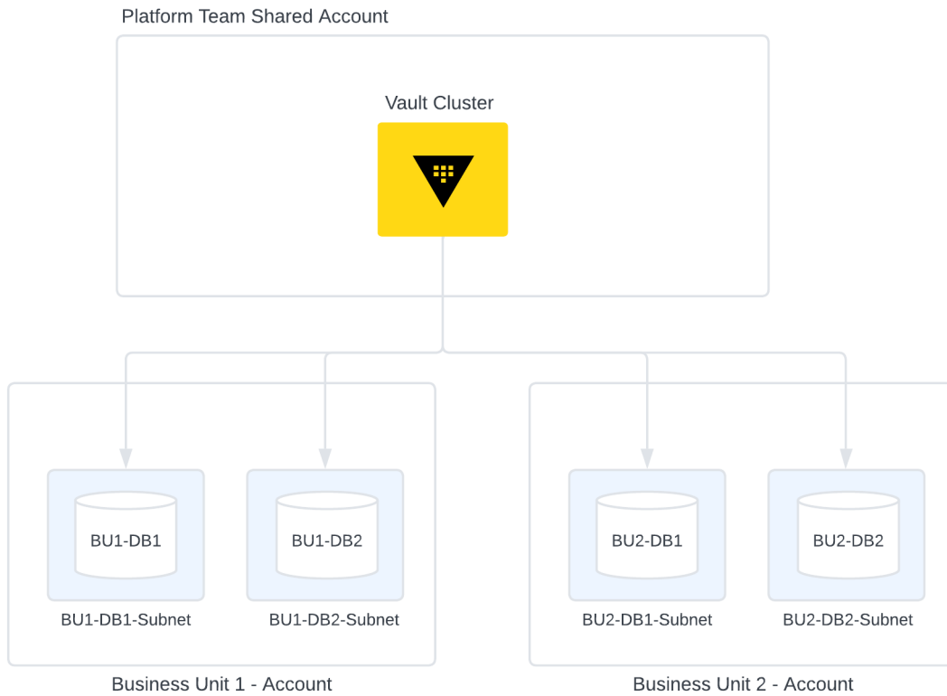
Figure 18: Dynamic Secret Network Considerations
