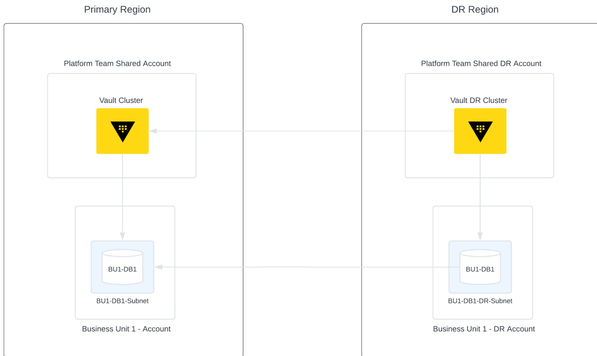
Figure 20: Dynamic Secret Network Considerations DR
