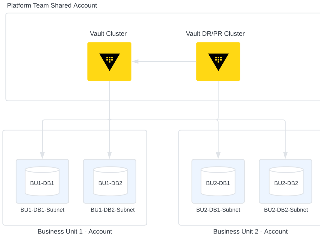
Figure 19: Dynamic Secret Network Considerations DR
