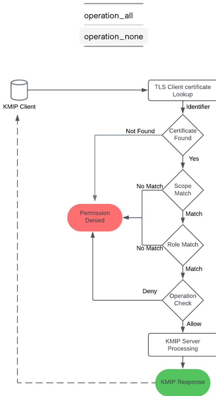
Figure 28: KMIP Client Flow Chart
