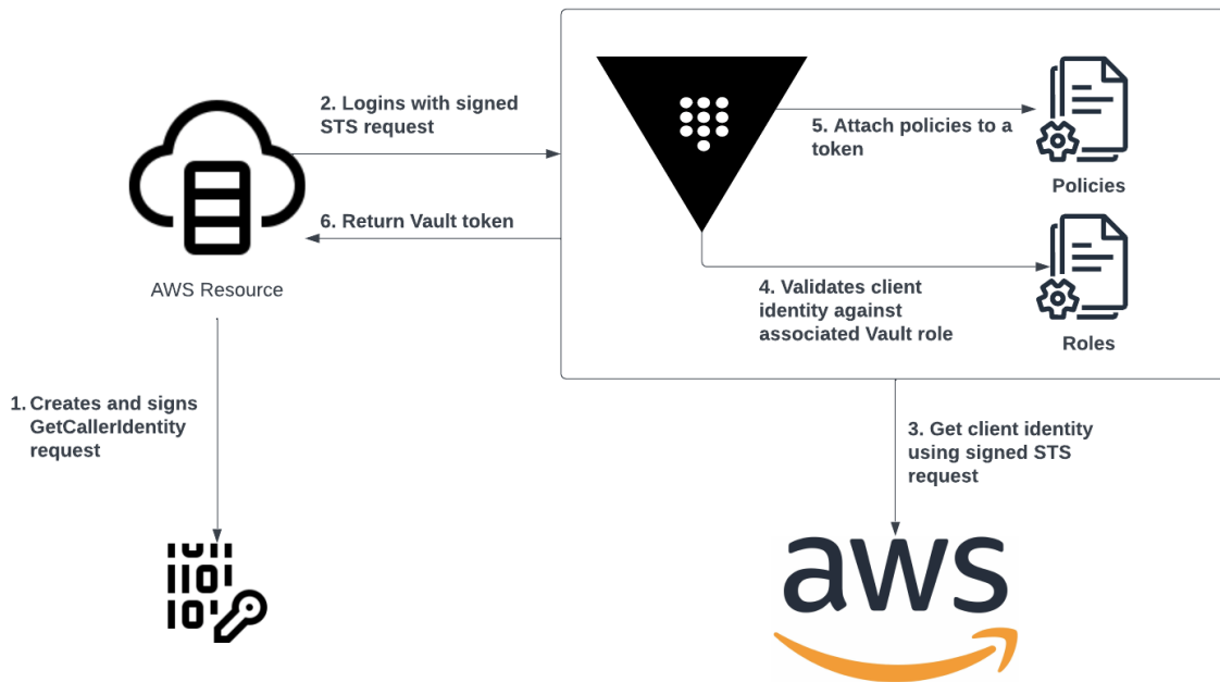
Figure 11: AWS auth method
