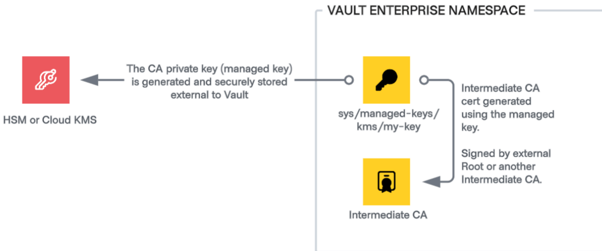
Figure 23: PKI managed keys with HSM or Cloud KMS
