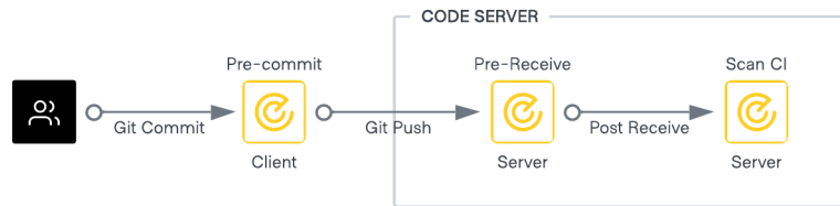
Figure 2: Vault Radar automation workflow
