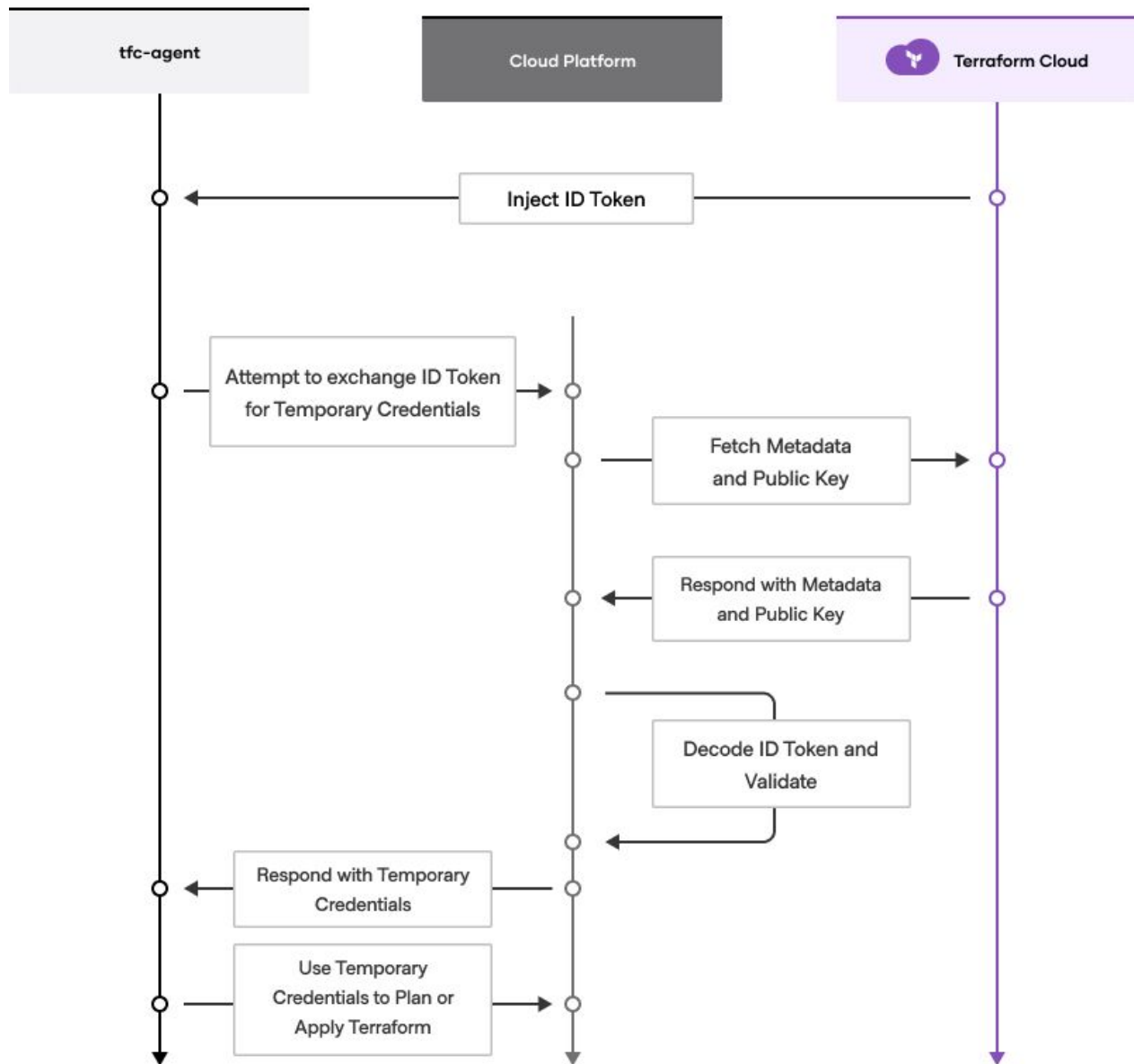
Figure 2: Workload identity with HCP Terraform
