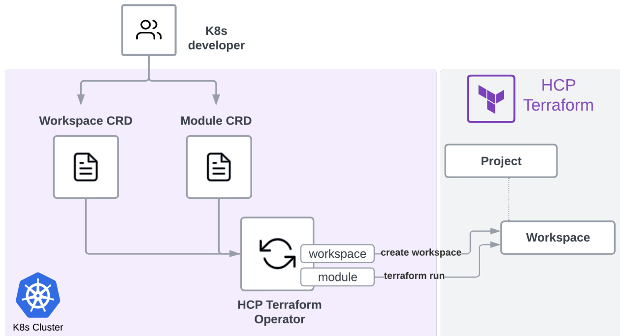
Figure 22: Kubernettes Consumption
