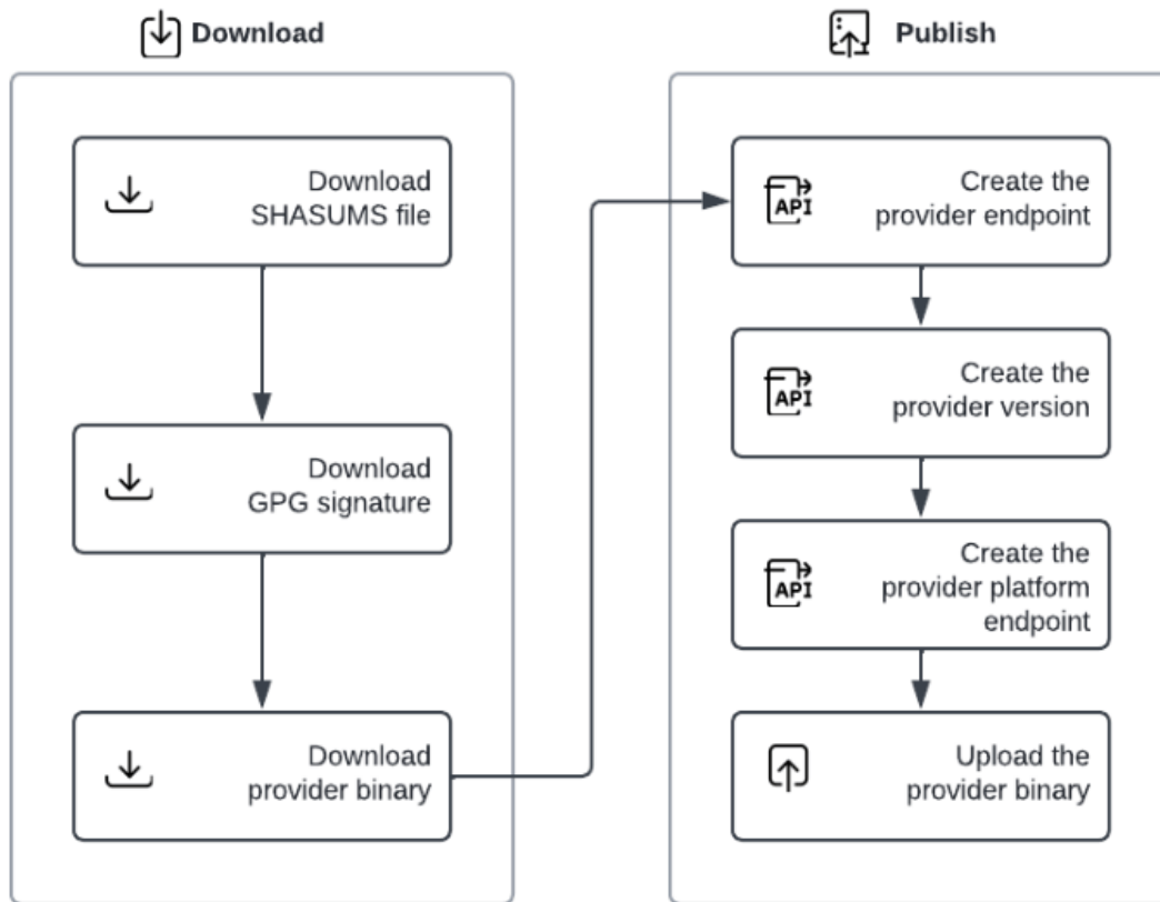
Figure 27: Publishing public providers or modules airgapped
