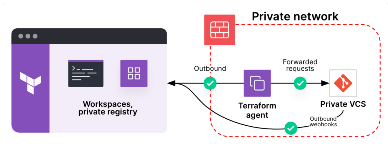
Figure 17: Private VCS
