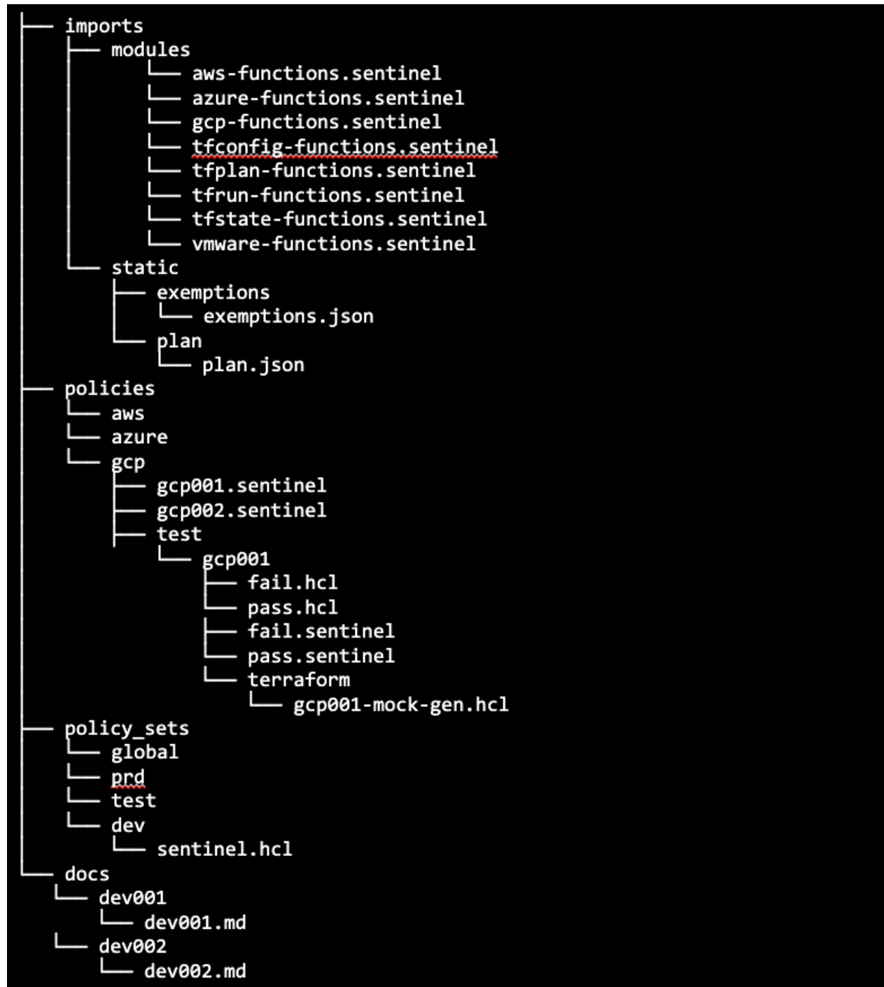
Figure 30: Repository Organization
