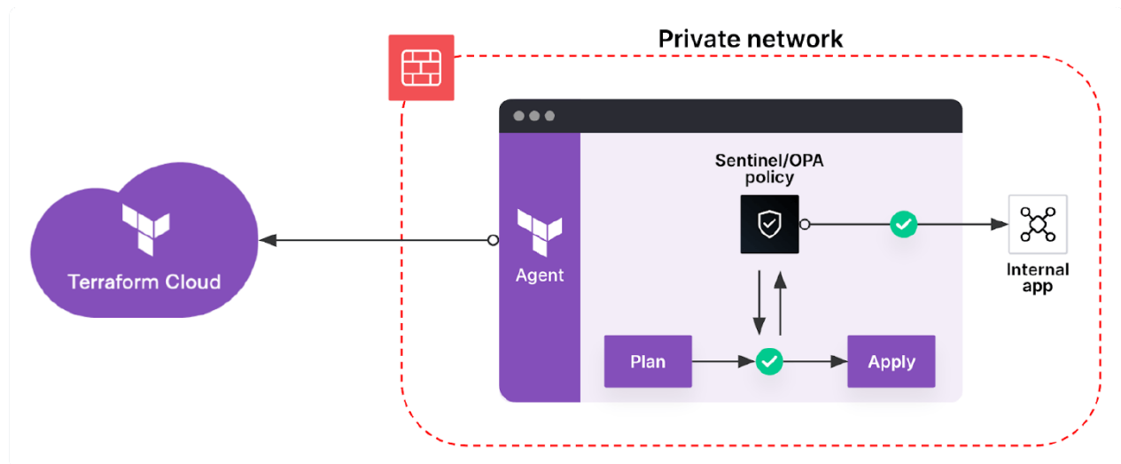
Figure 18: Sentinel Policies
