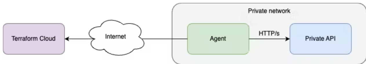
Figure 16: Agent Connections
