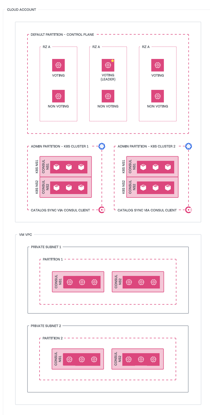
Figure 1: Consul AWS Architecture
