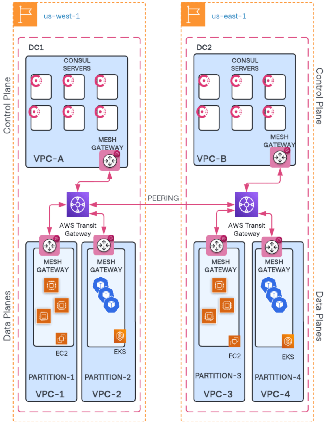
Figure 9: Consul multi-cluster recommended architecture
