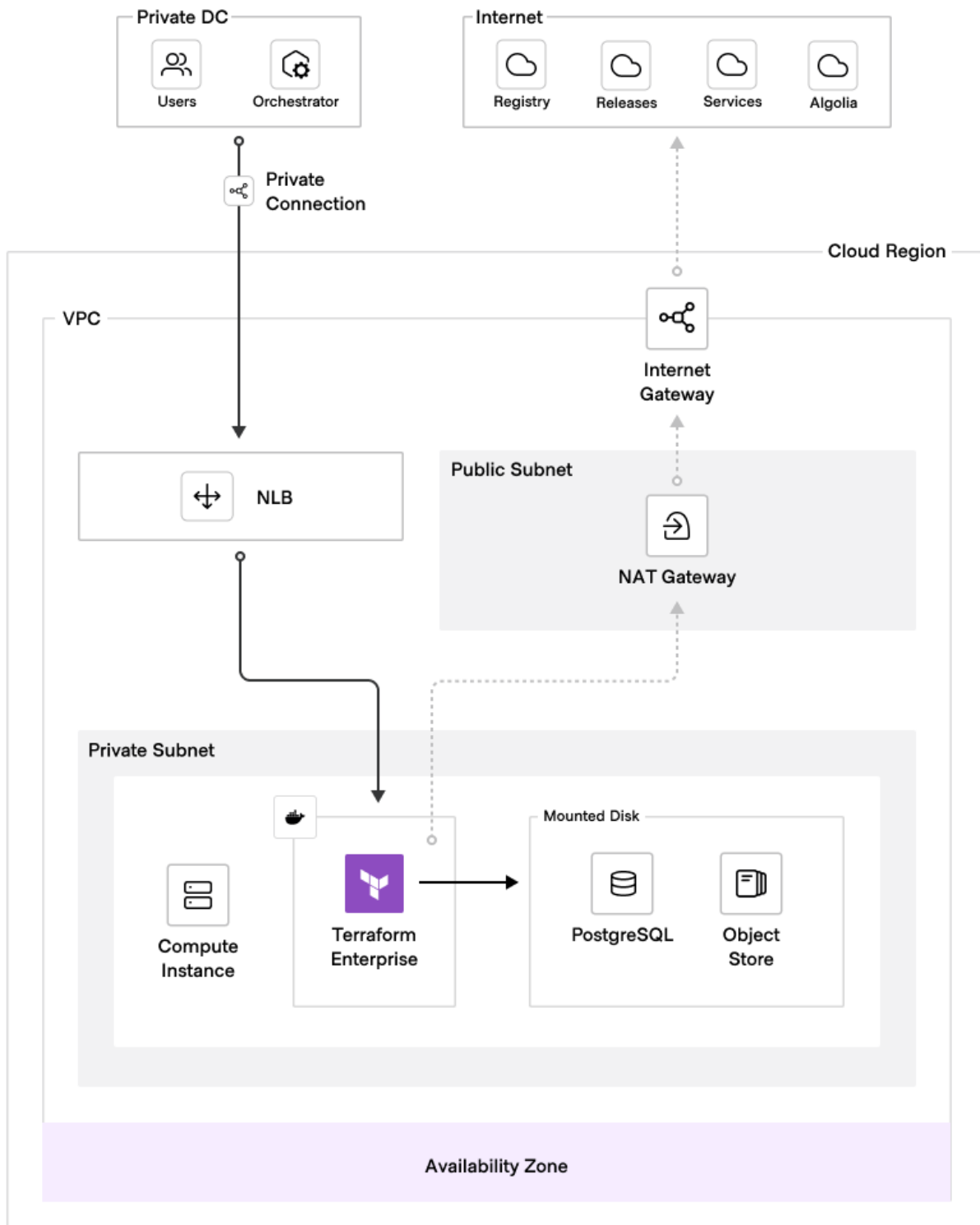
Figure 1: Terraform disk operational mode
