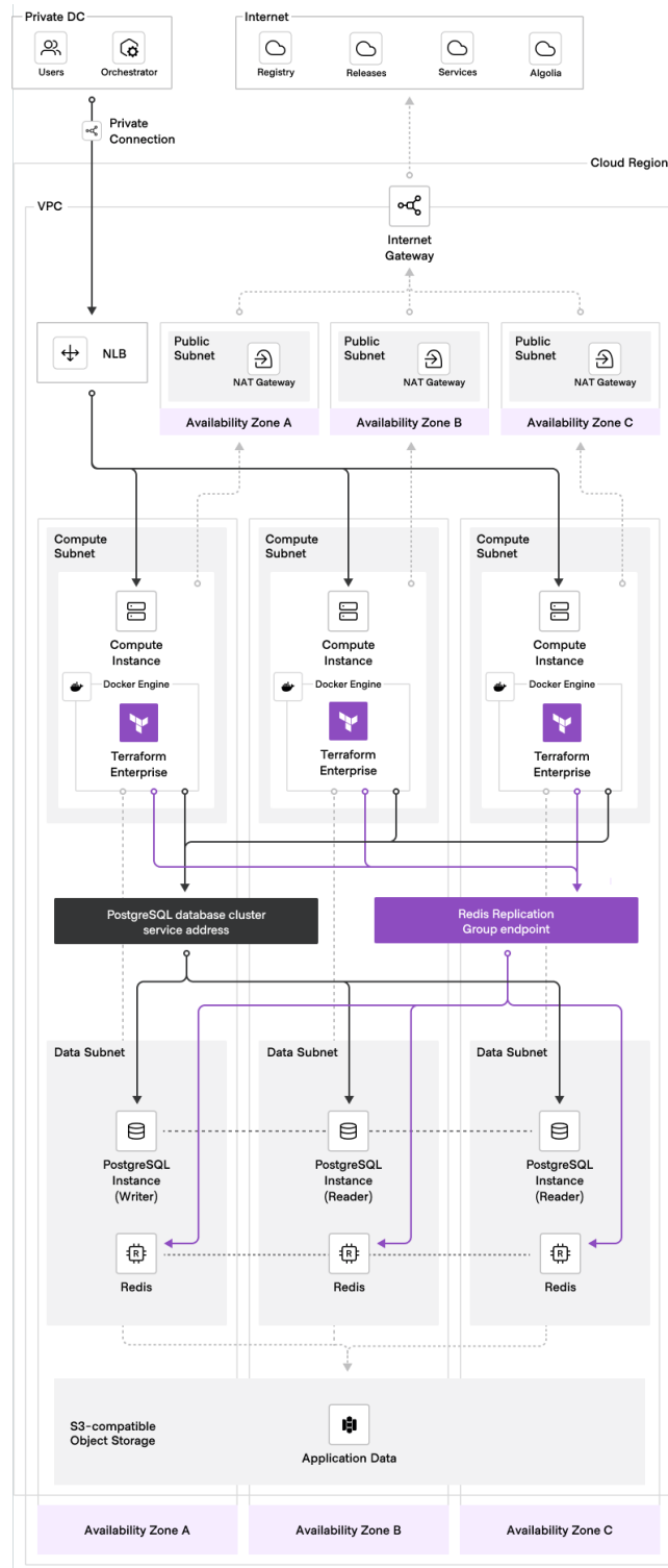
Figure 3: active-active mode operational mode
