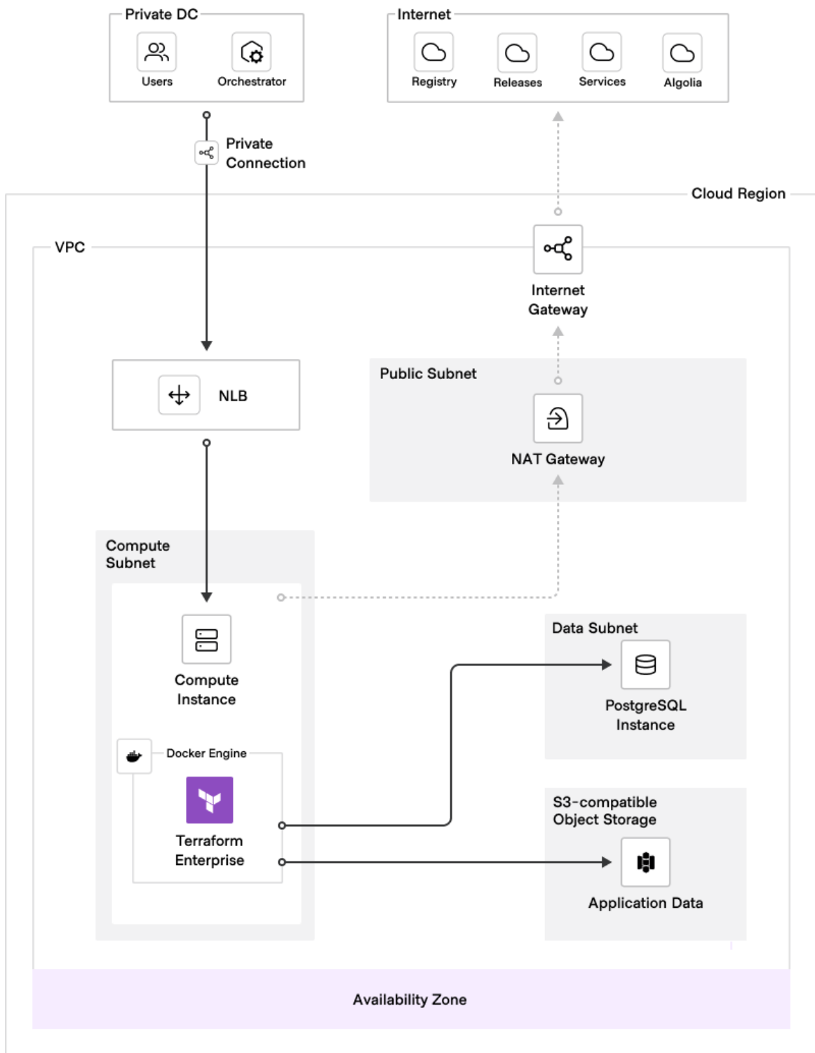
Figure 2: external mode operational mode
