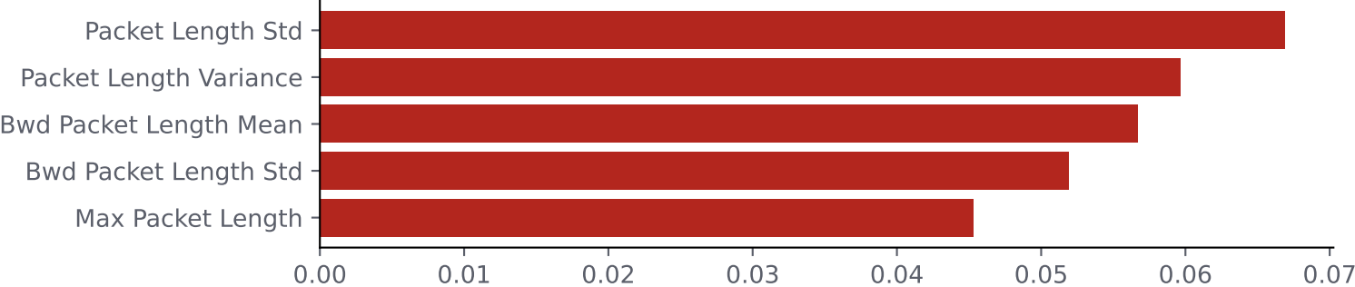
Top feature importances (leakage_screen)
