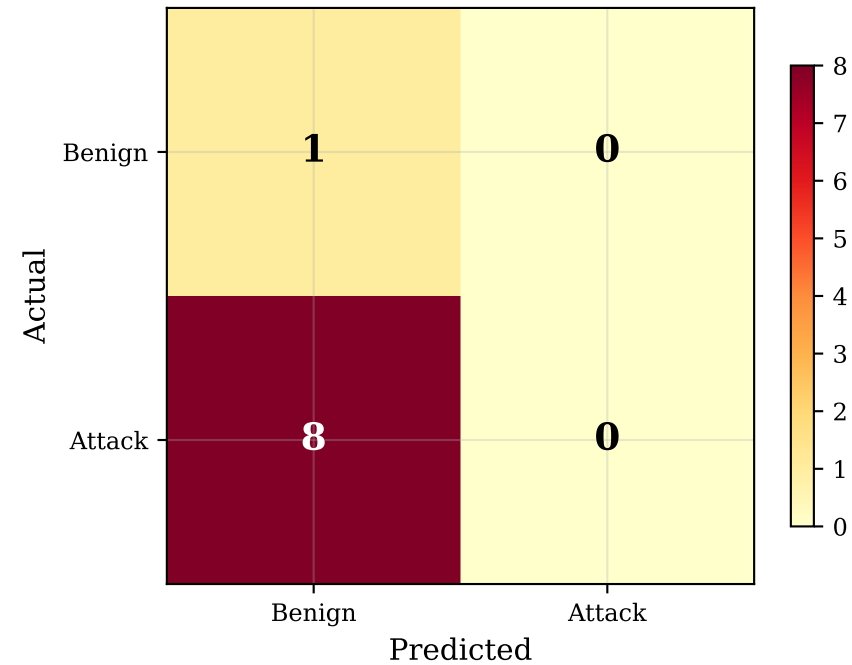
B1+B2+B3 (Acc: 11.1%, F1: nan)
