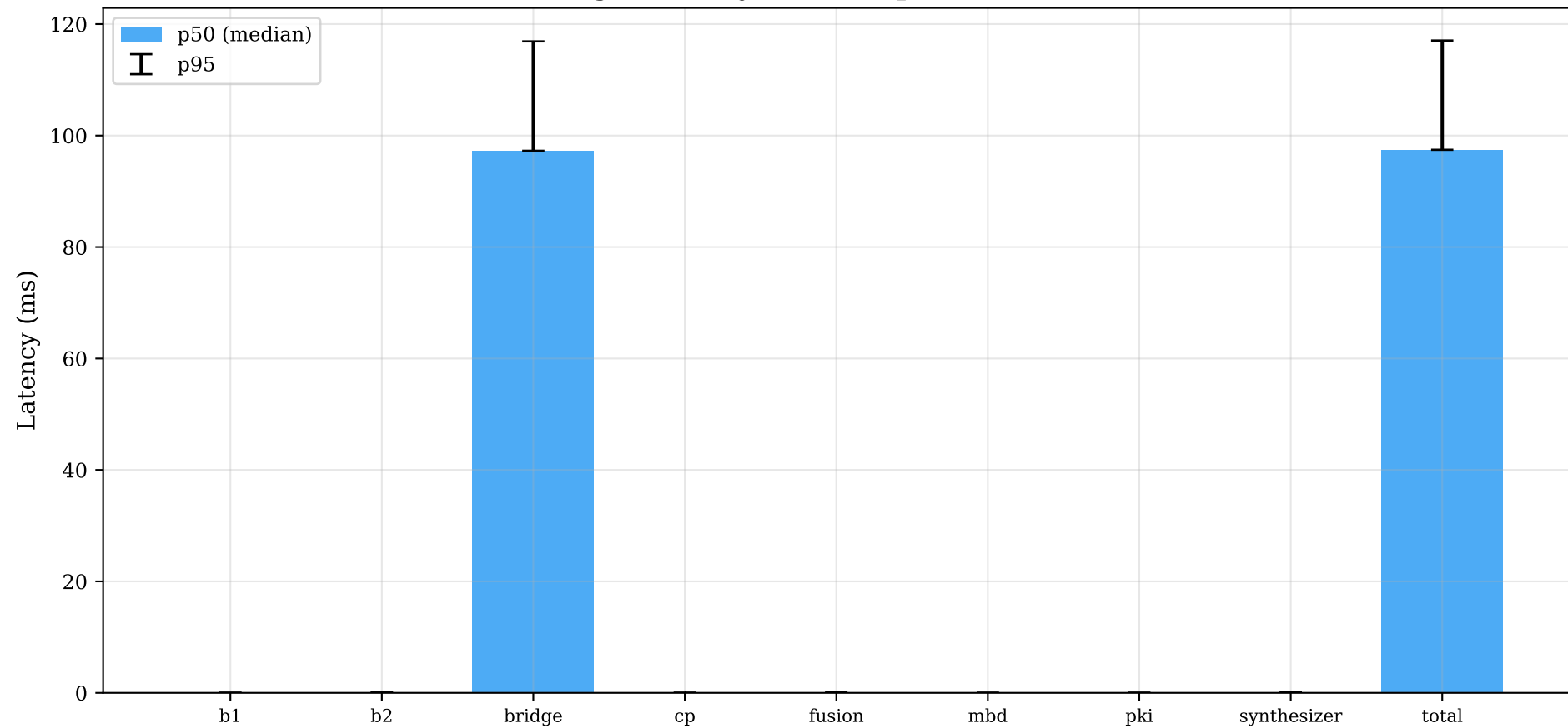
Per-Stage Latency — Full Pipeline (B1+B2+B3)
