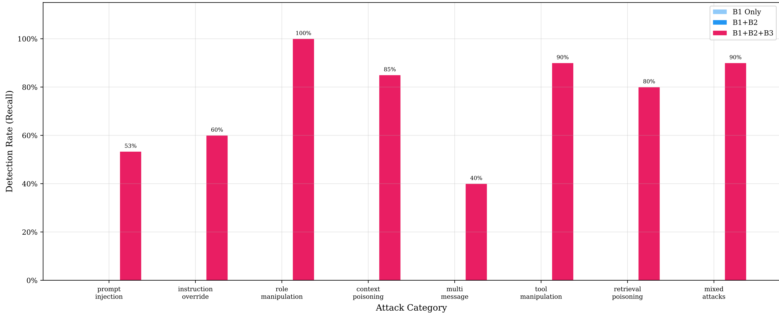
Detection Rate by Attack Category — B3 Contribution
