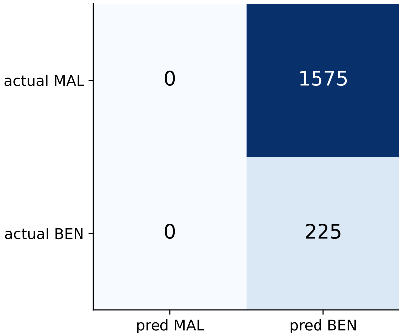
Confusion Matrix (full stack)
