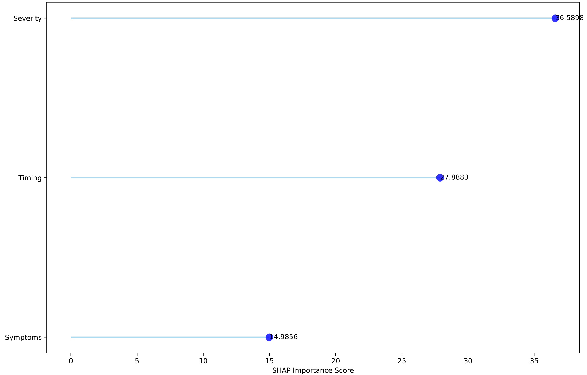
Clinical Variables Associated with Bifidobacterium.pseudocatenulatum Abundance
