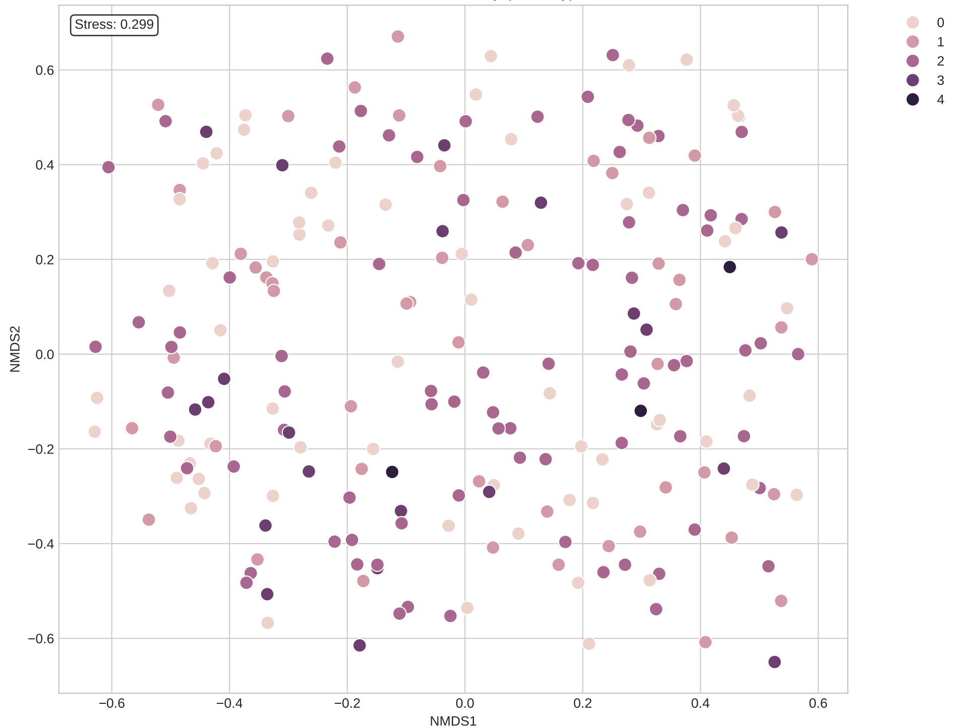
NMDS of Beta Diversity (Severity)
