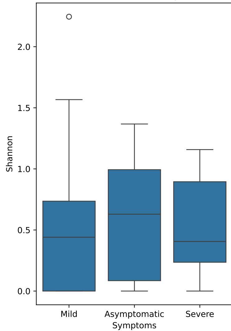
Shannon Diversity
