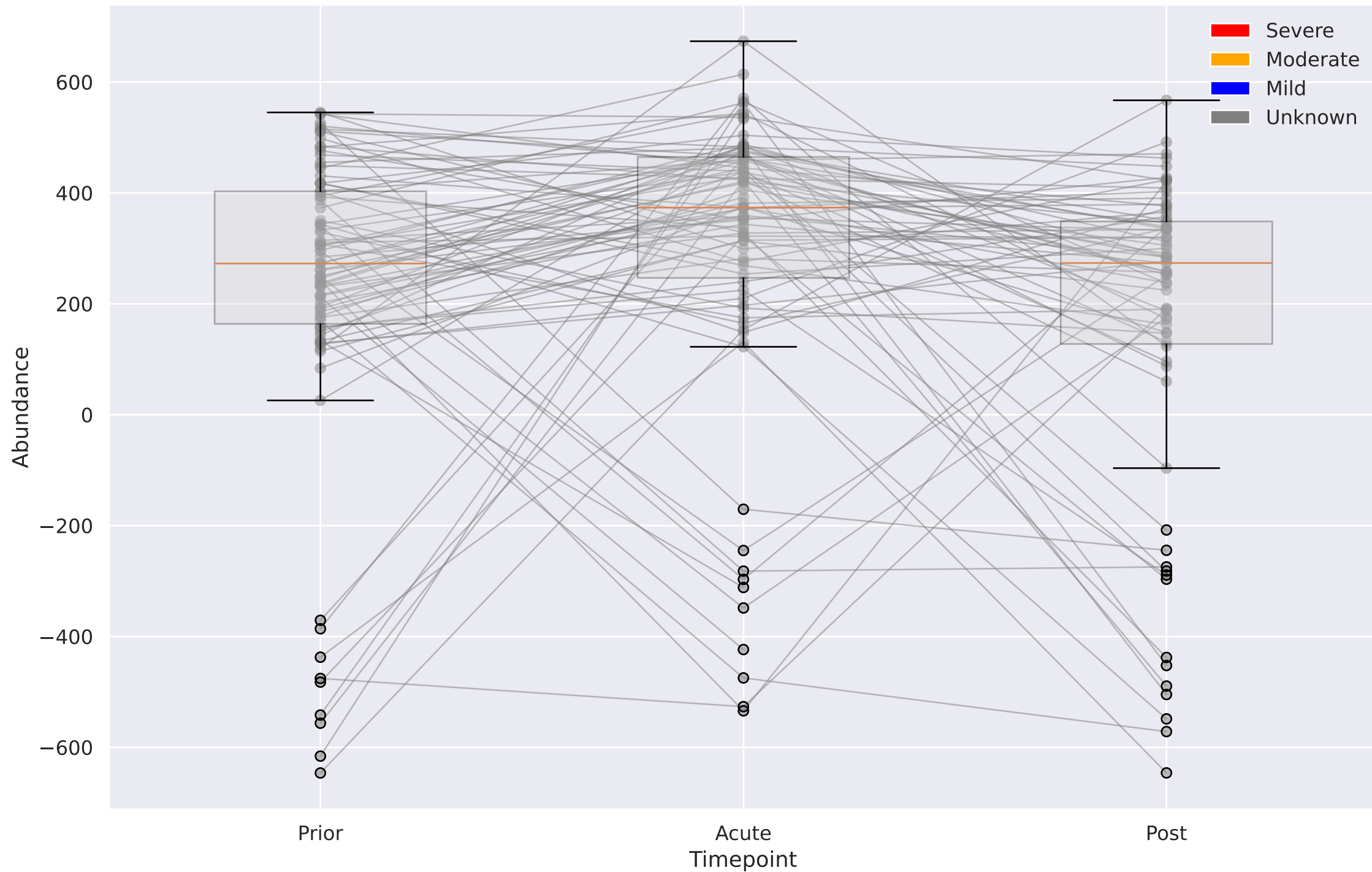
Moraxella.catarrhalis Abundance Trajectory by Subject
