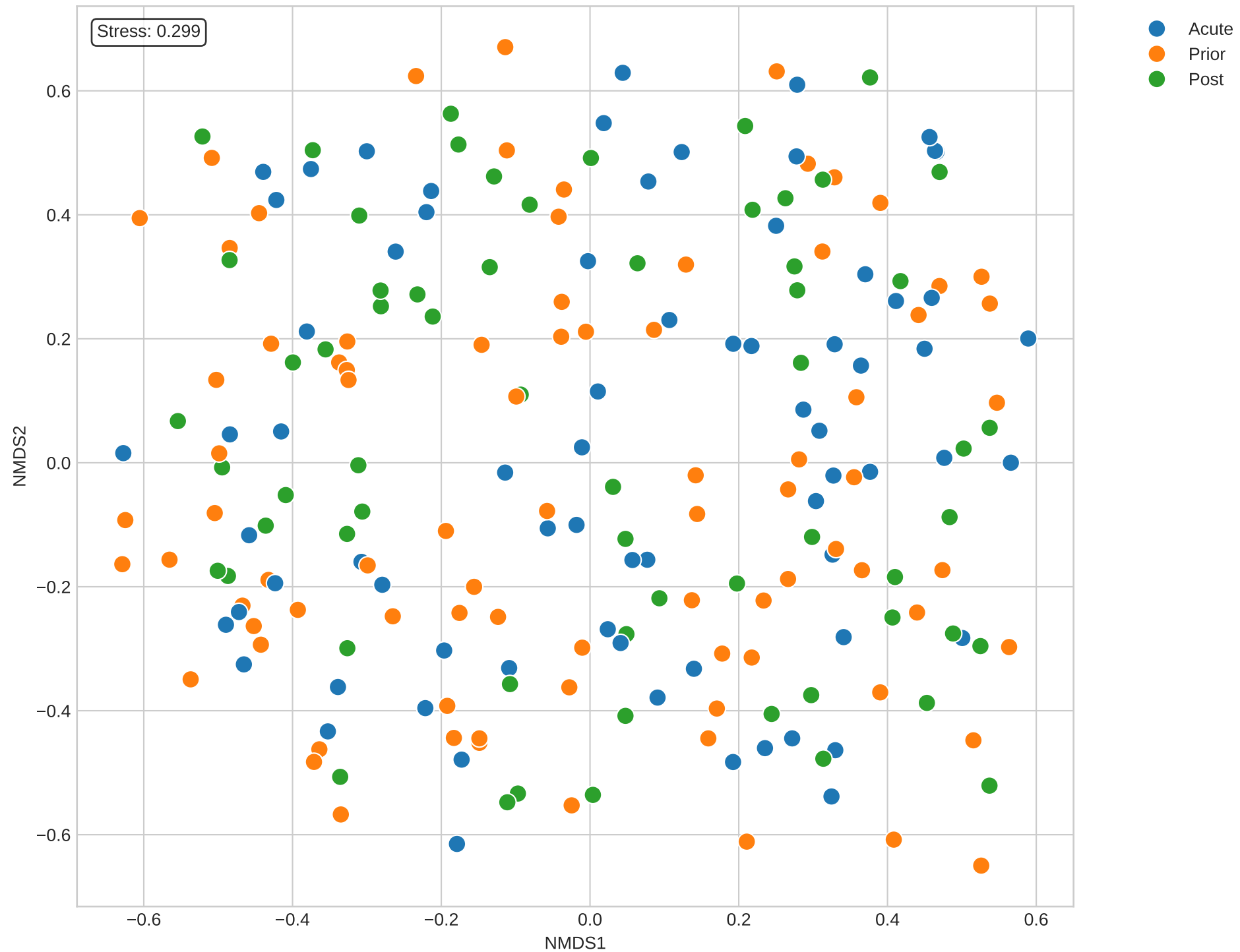
NMDS of Beta Diversity (Timing)
