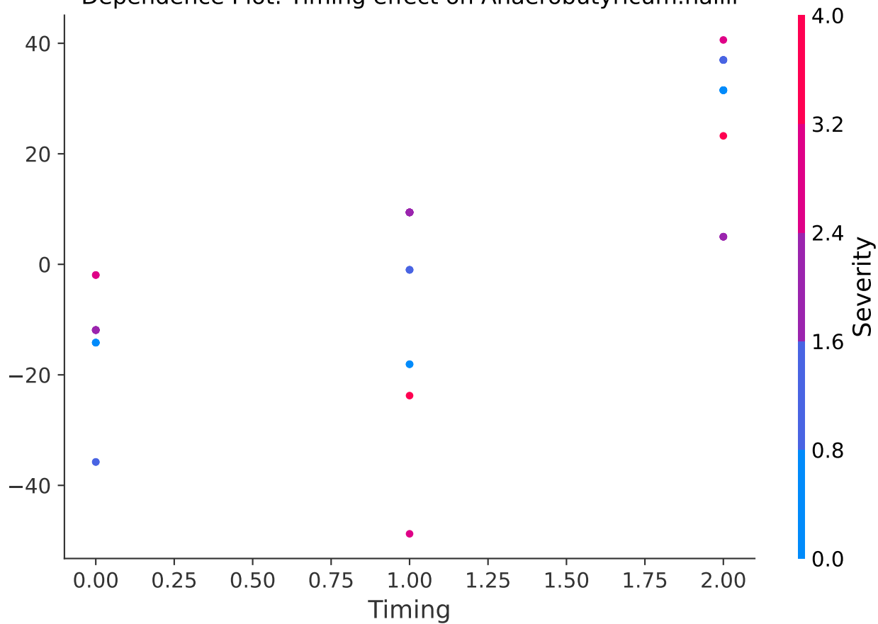
Dependence Plot: Timing effect on Anaerobutyricum.hallii
