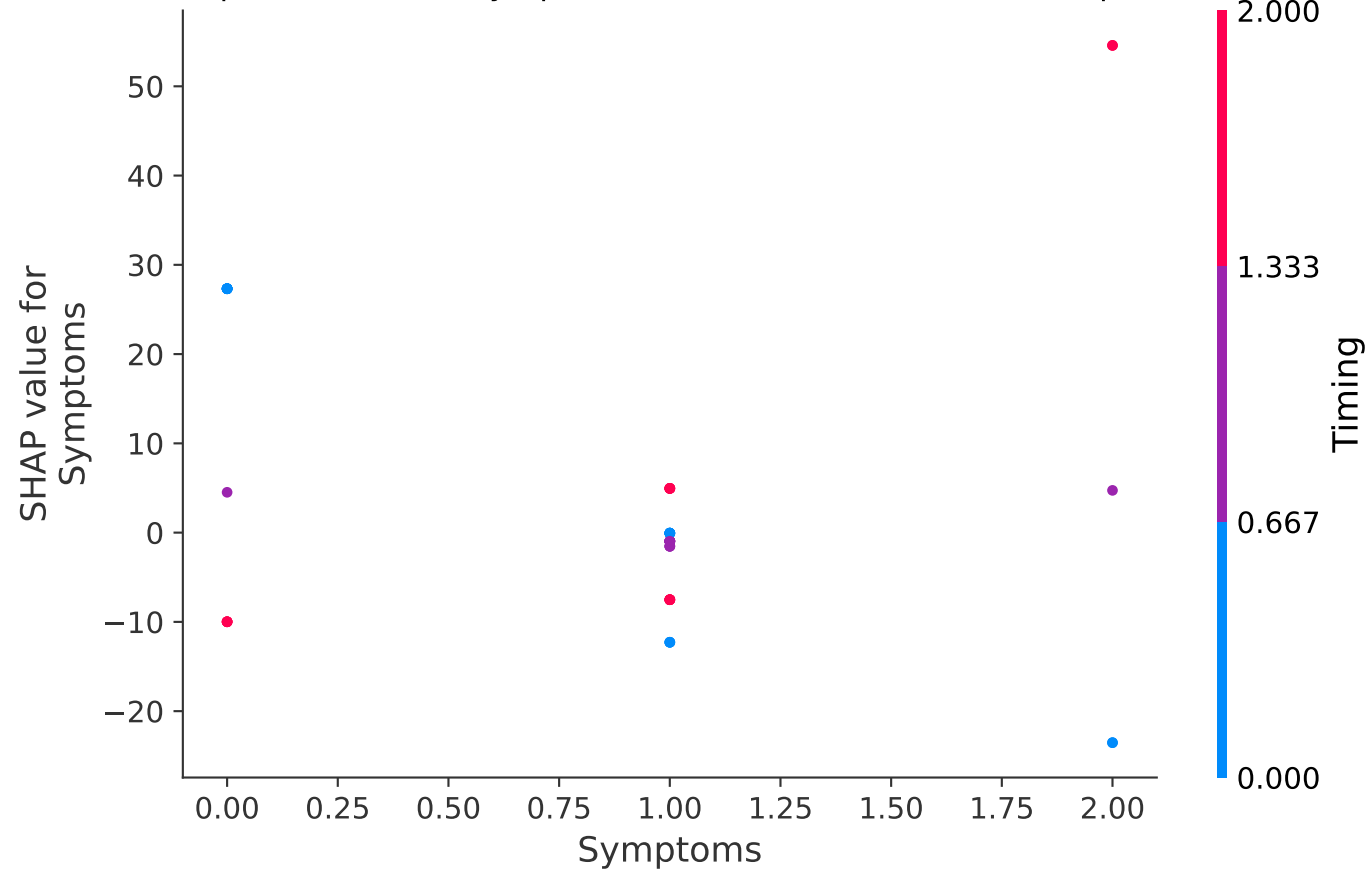
Dependence Plot: Symptoms effect on Ruminococcus.torques
