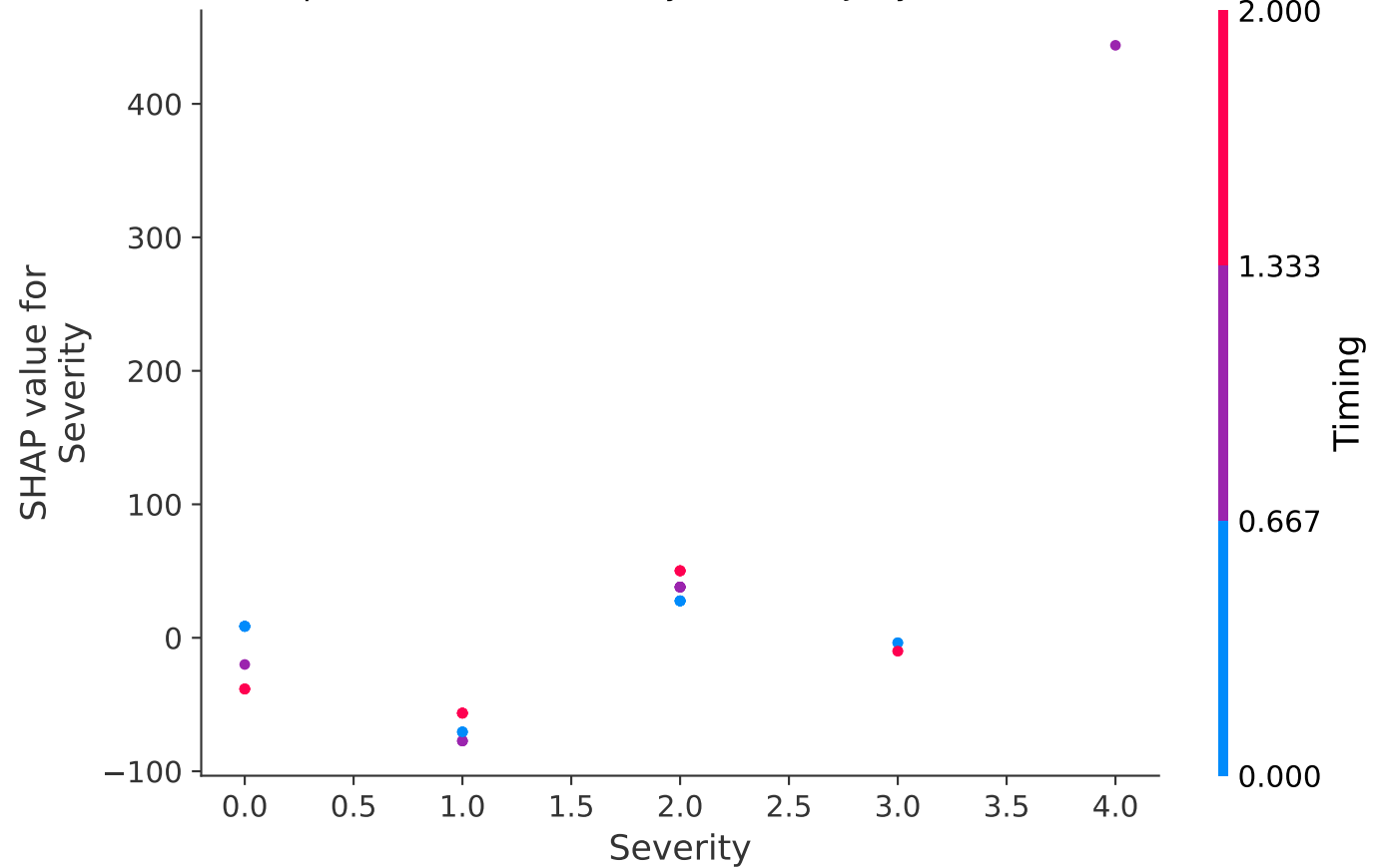
Dependence Plot: Severity effect on Jouyvirus.ev207
