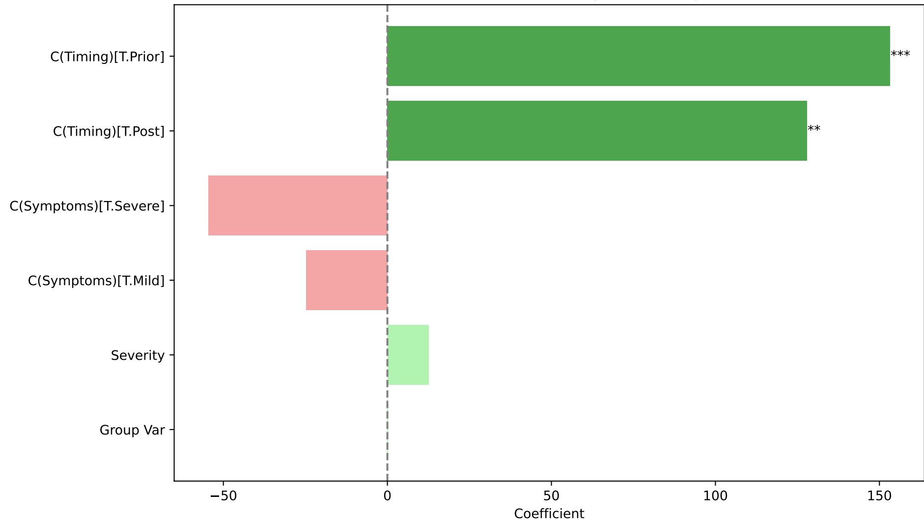
Mixed Model Coefficients: Bradyrhizobium.sp.41S5
