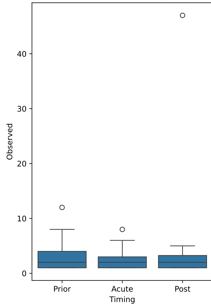
Observed Diversity
