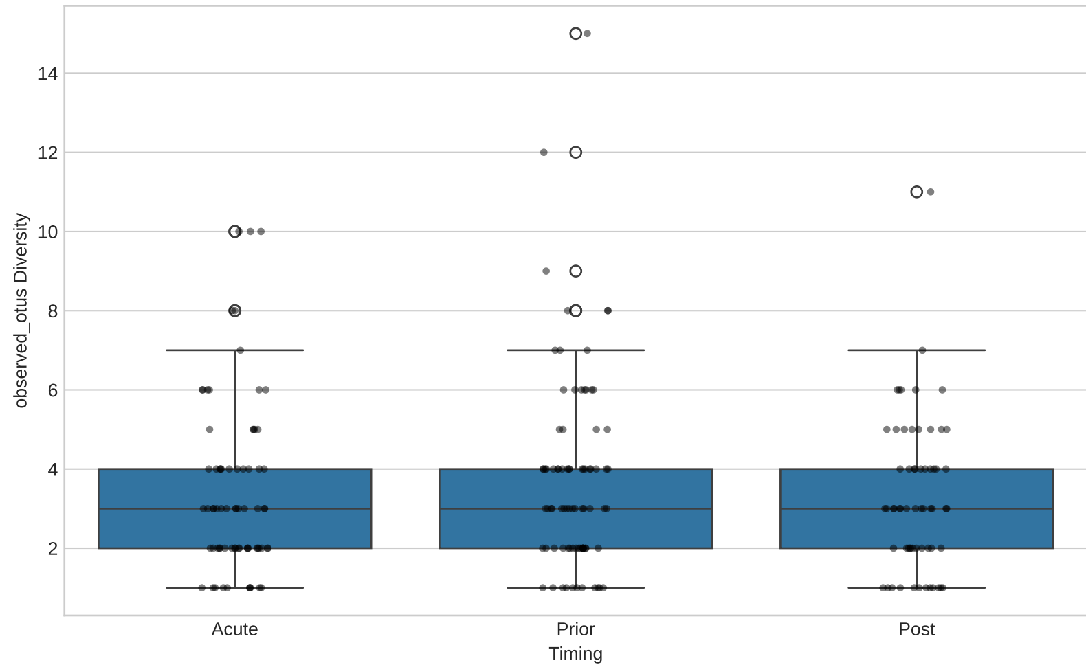
observed_otus Diversity by Timing
