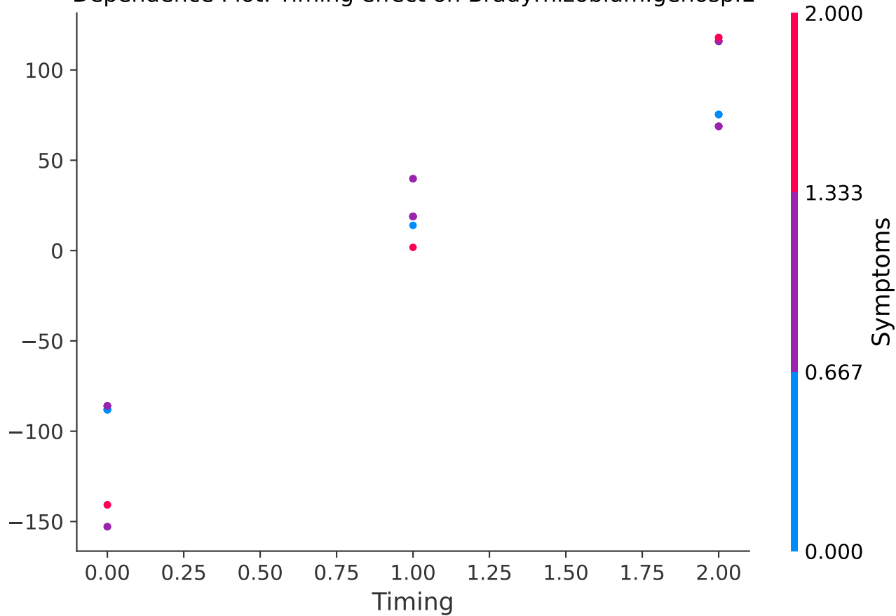
Dependence Plot: Timing effect on Bradyrhizobium.genosp.L
