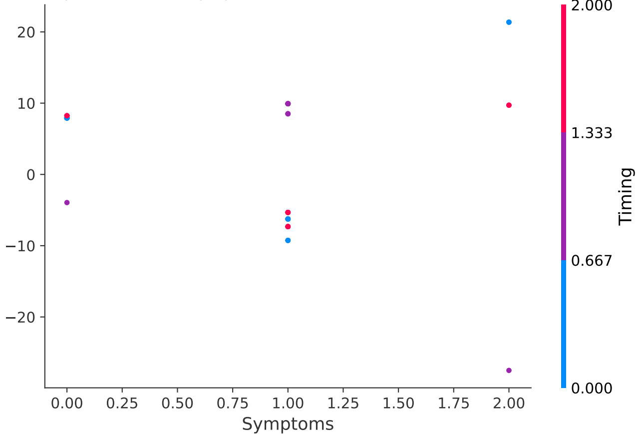
Dependence Plot: Symptoms effect on Collinsella.aerofaciens
