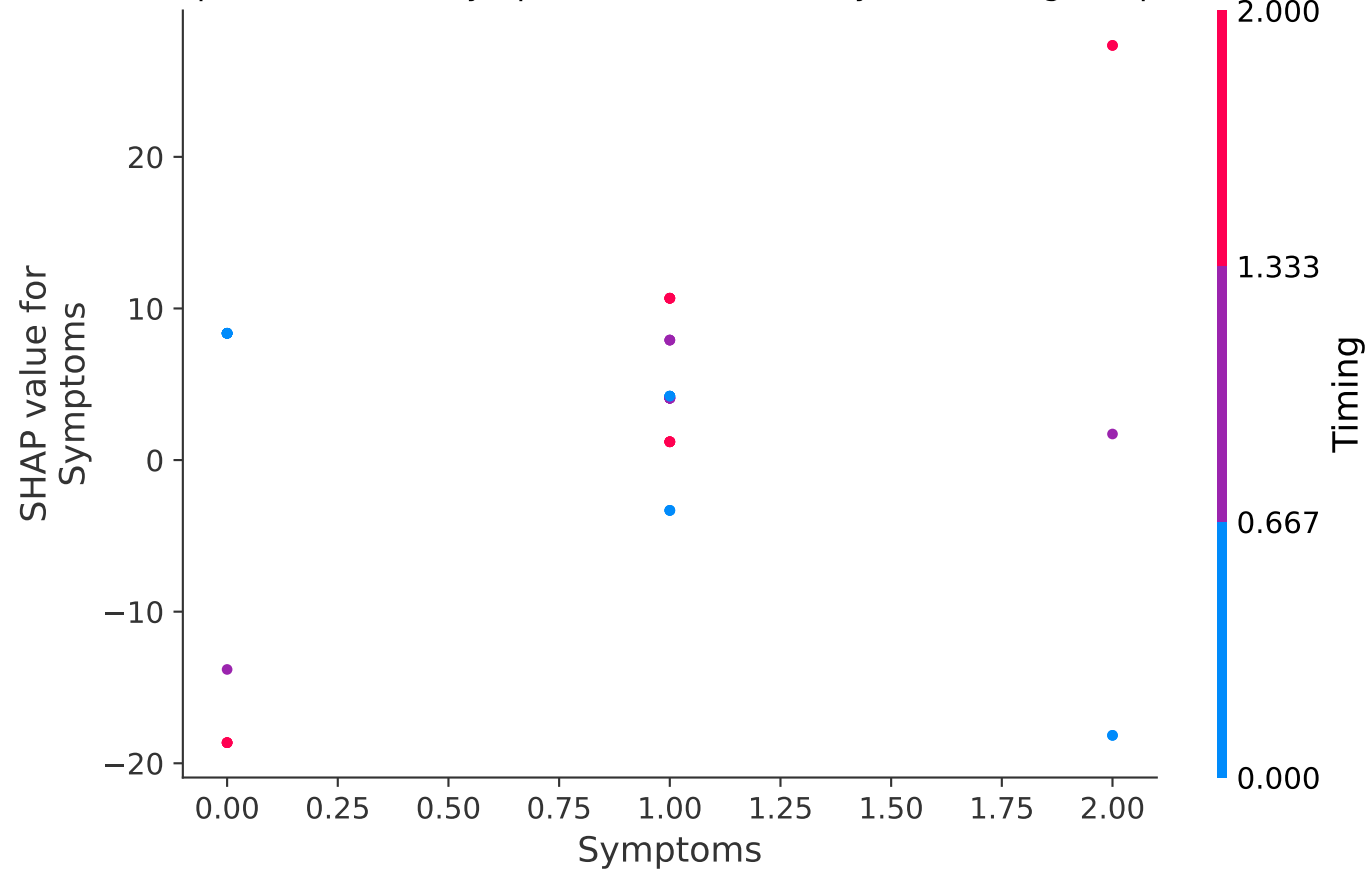
Dependence Plot: Symptoms effect on Bradyrhizobium.genosp.L
