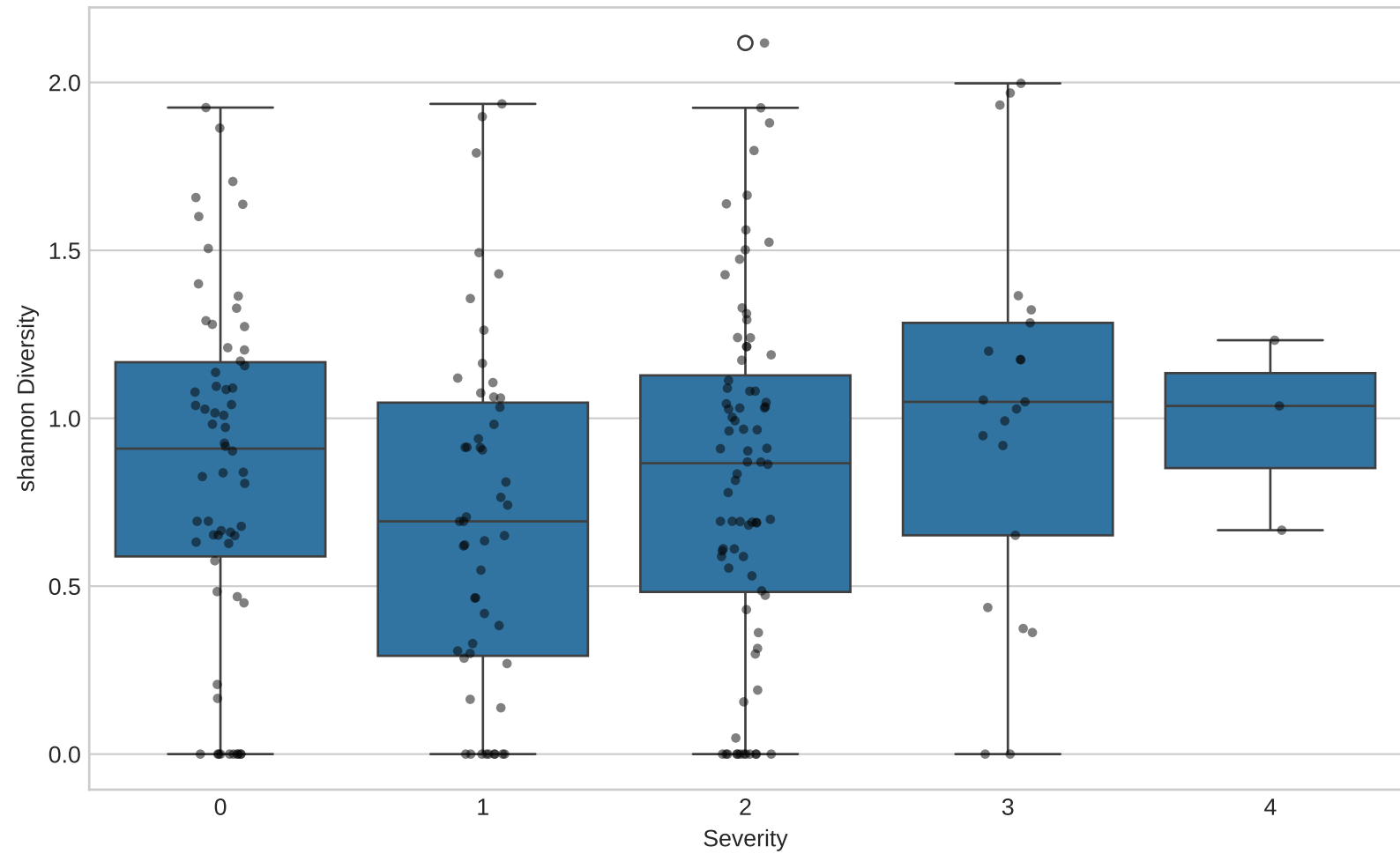
shannon Diversity by Severity
