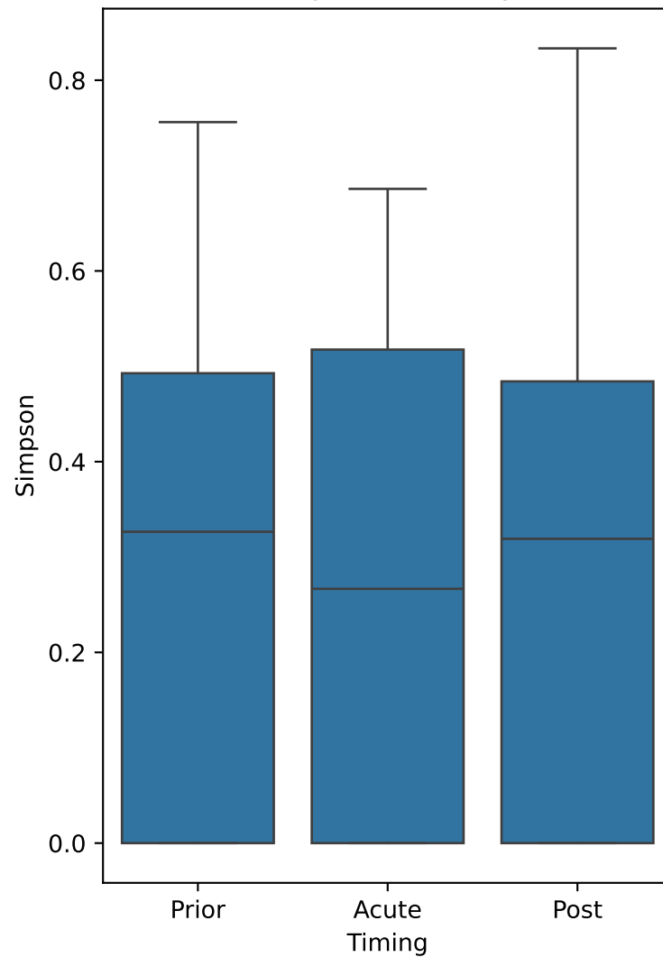
Simpson Diversity
