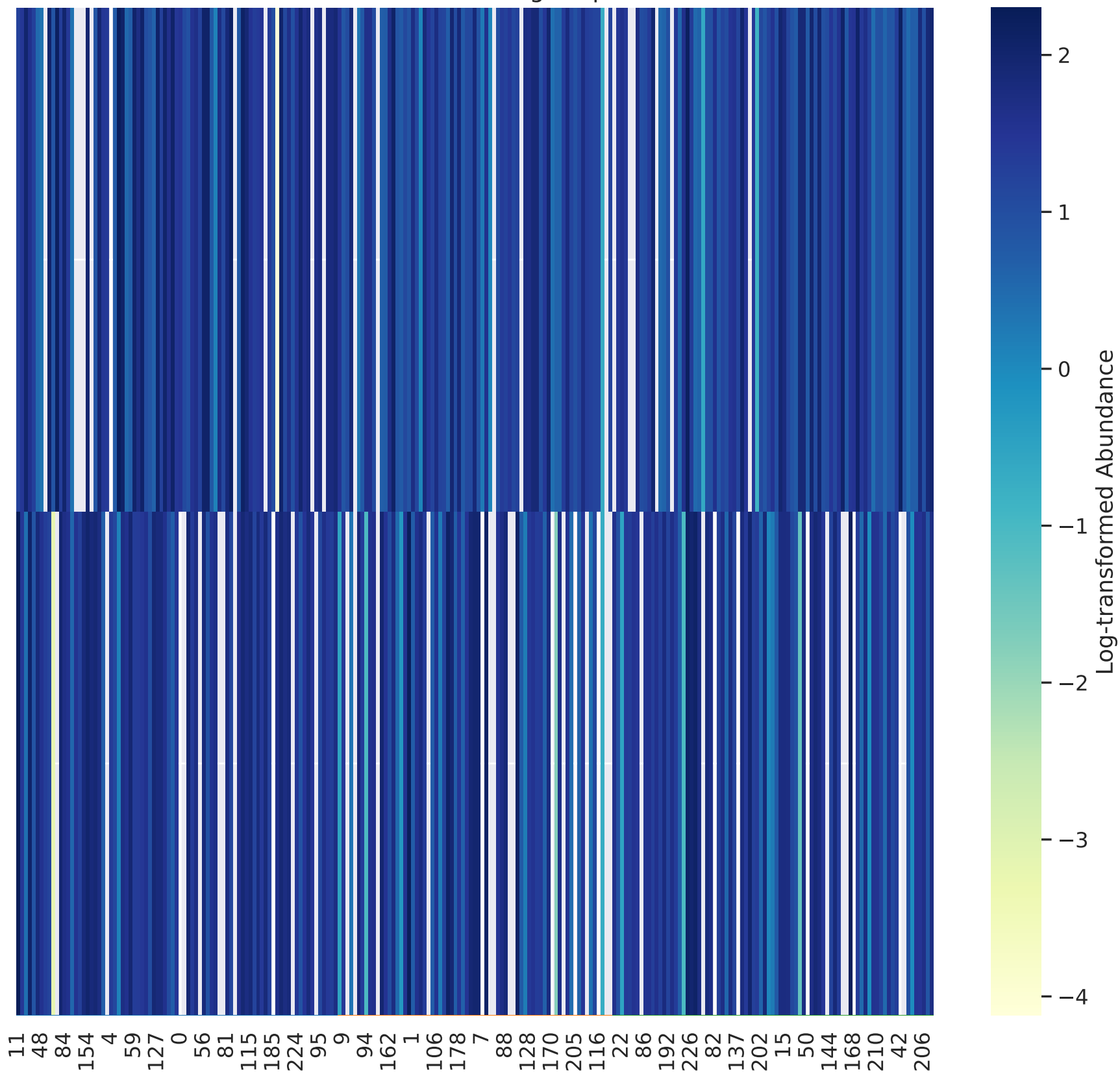
Co-occurrence of Target Species
