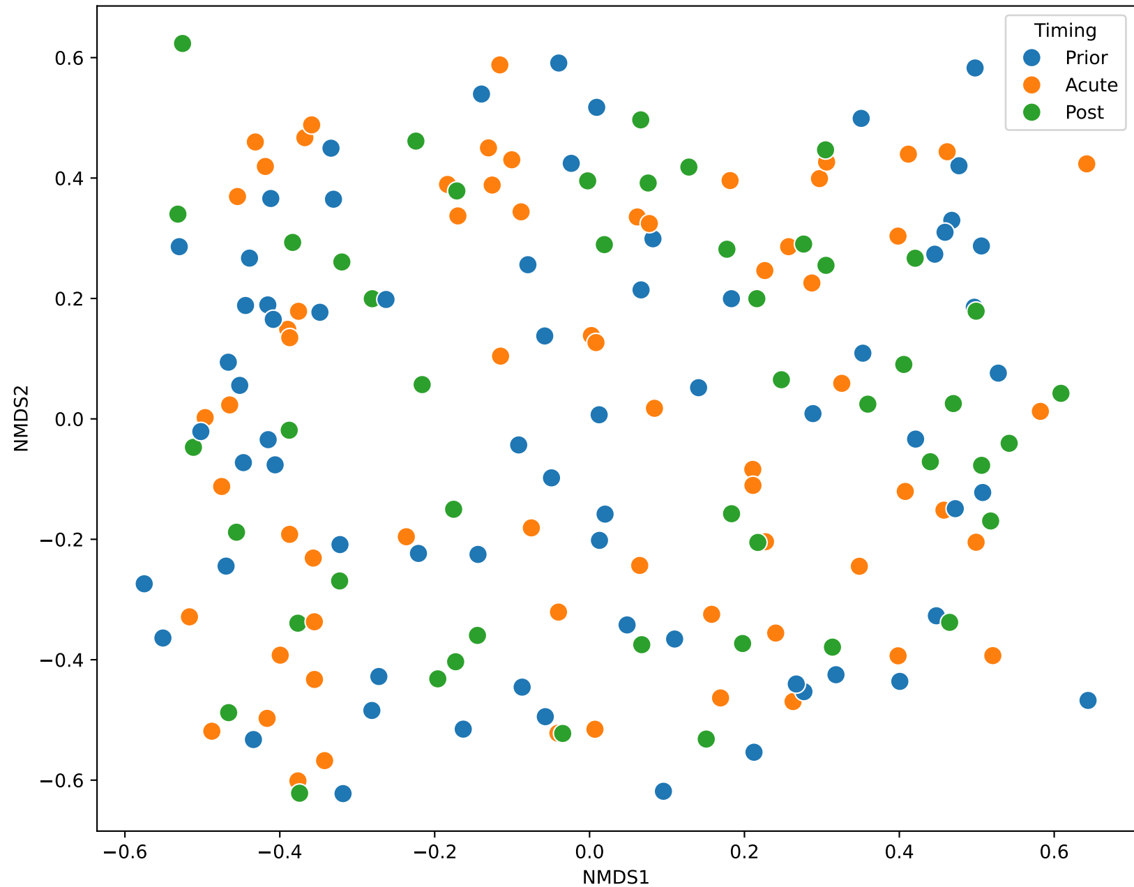
NMDS of Beta Diversity (Timing)
