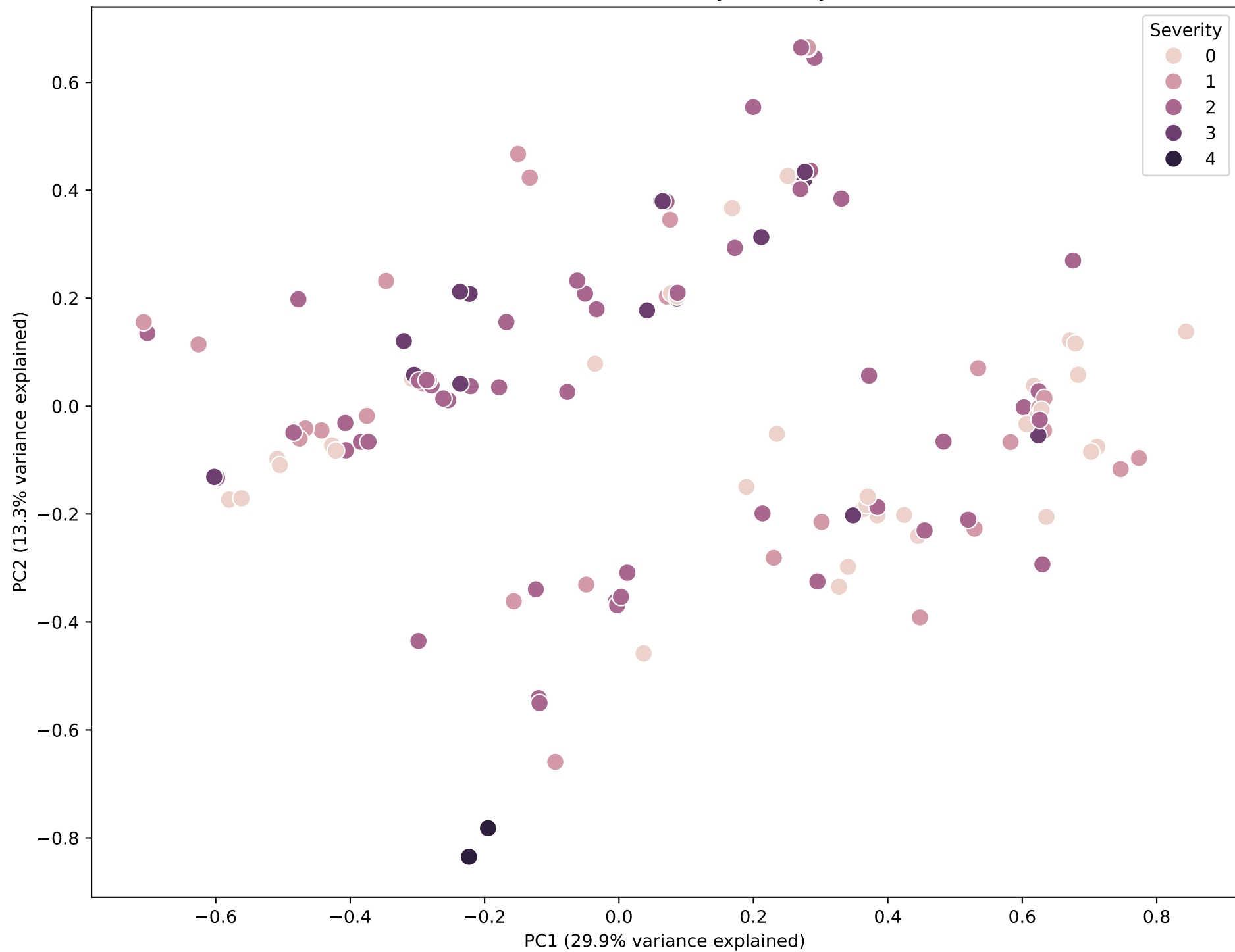
PCoA of Beta Diversity (Severity)
