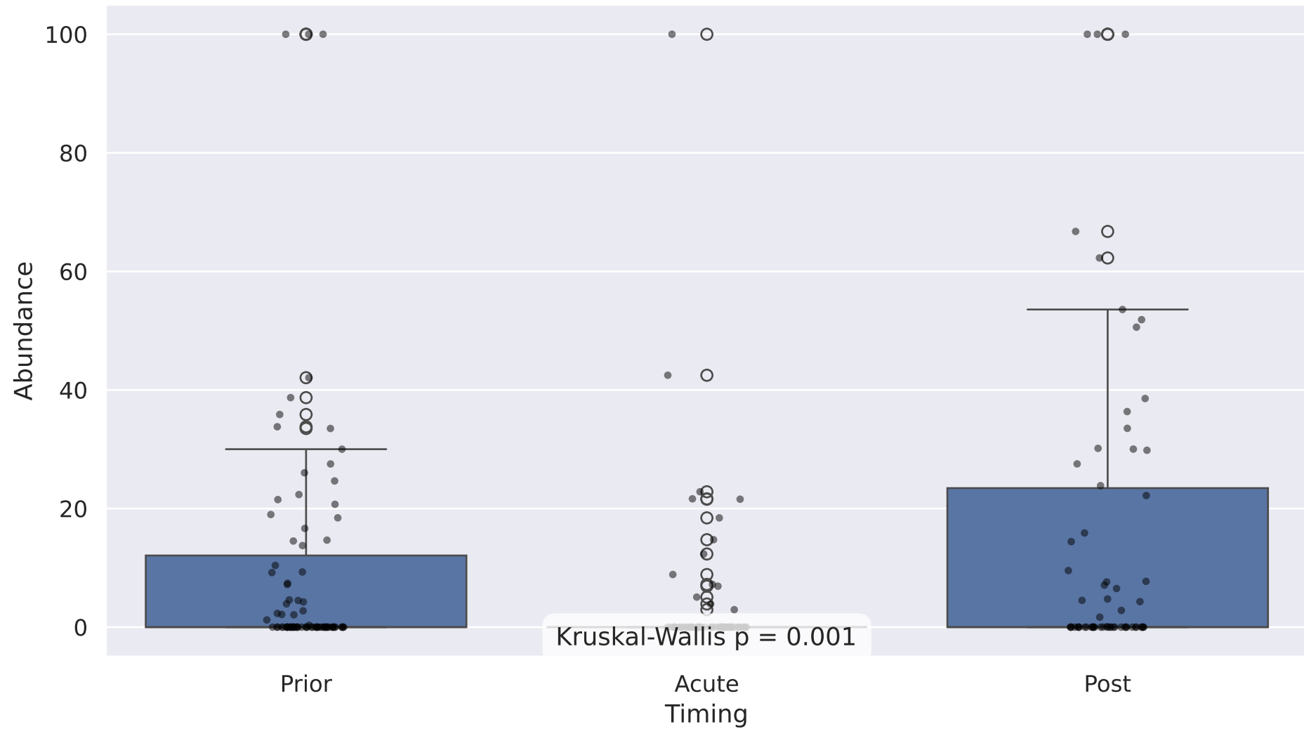
Bacteria: Cutibacterium acnes Abundance Across Time Points
