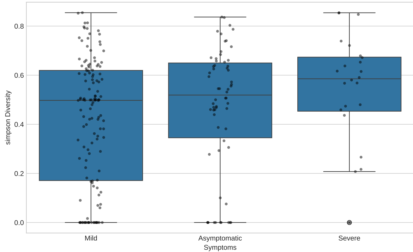
simpson Diversity by Symptoms
