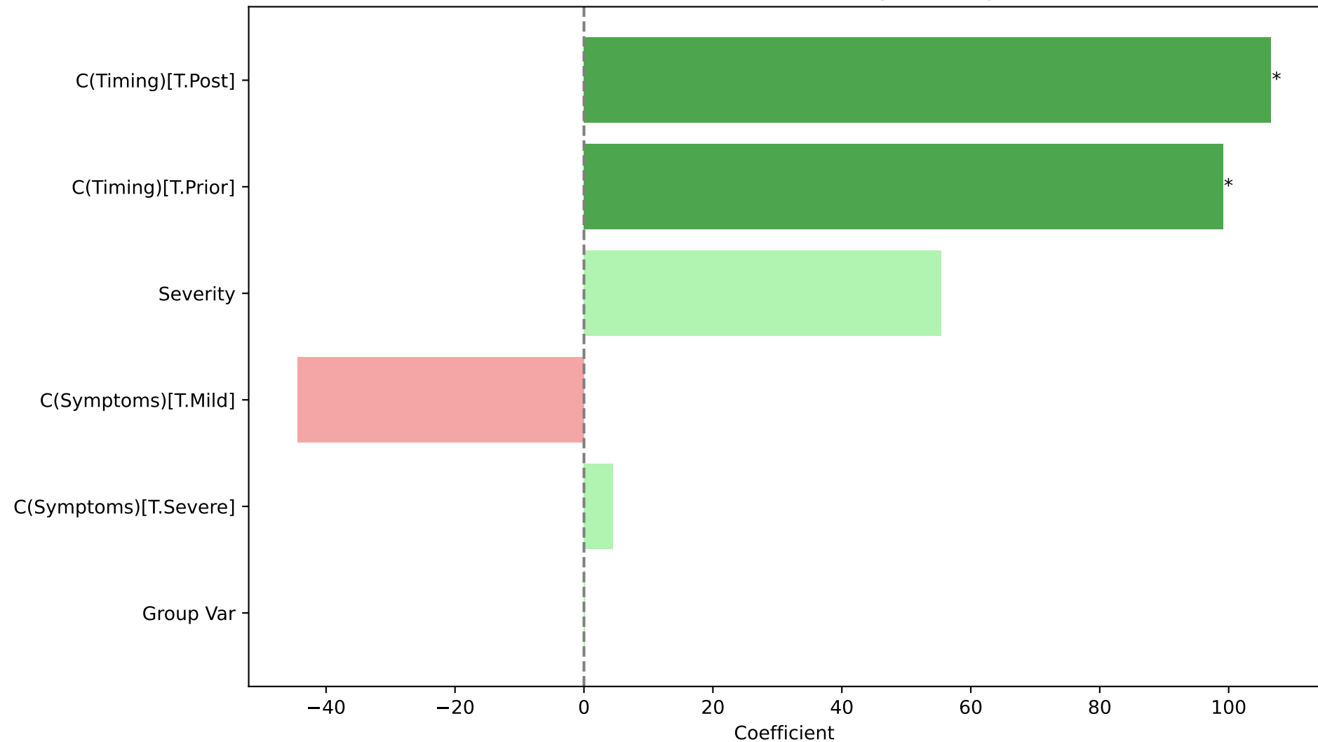
Mixed Model Coefficients: Segatella.copri
