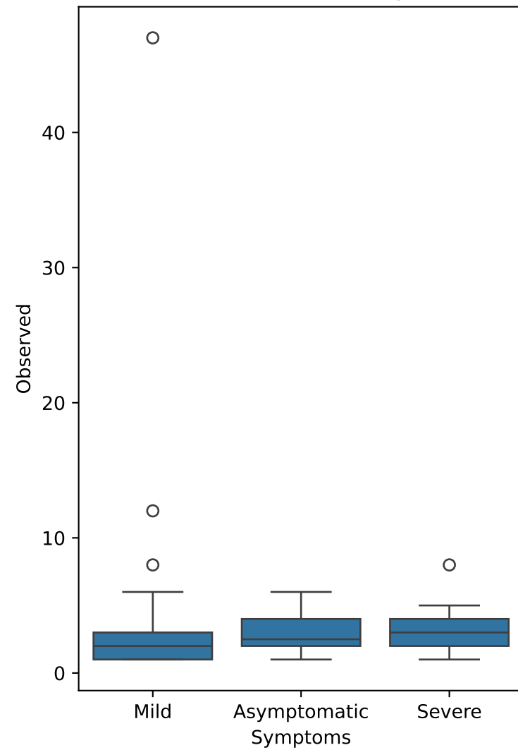
Observed Diversity
