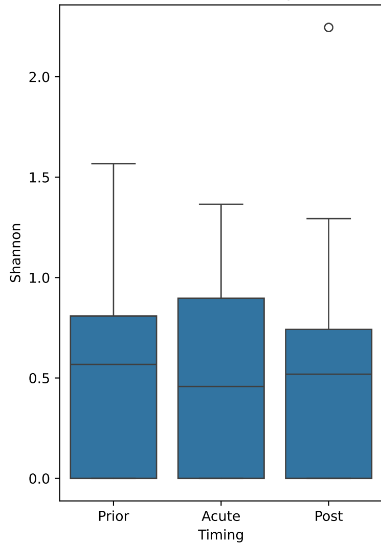
Shannon Diversity
