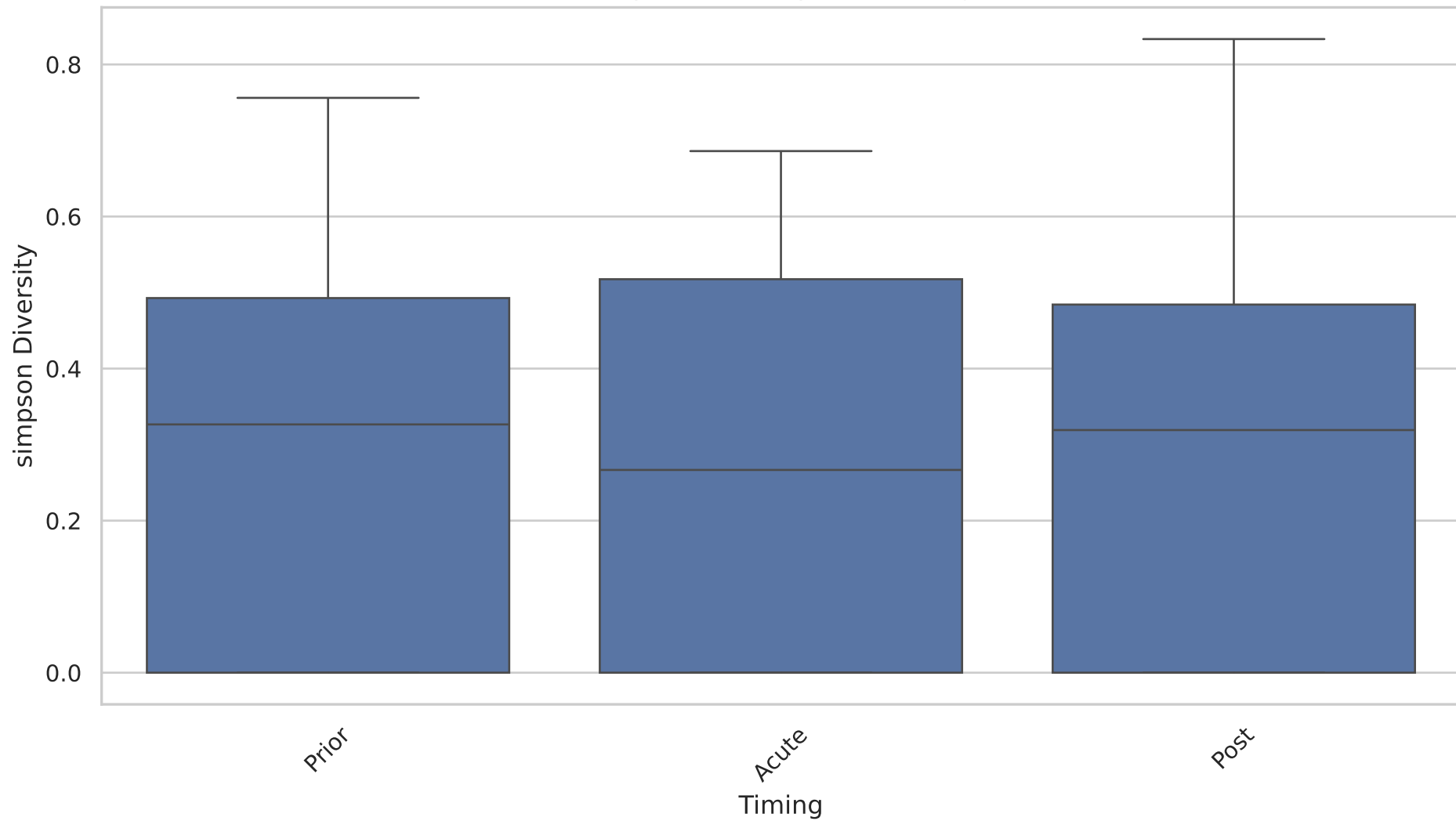
simpson Diversity Over Timing
