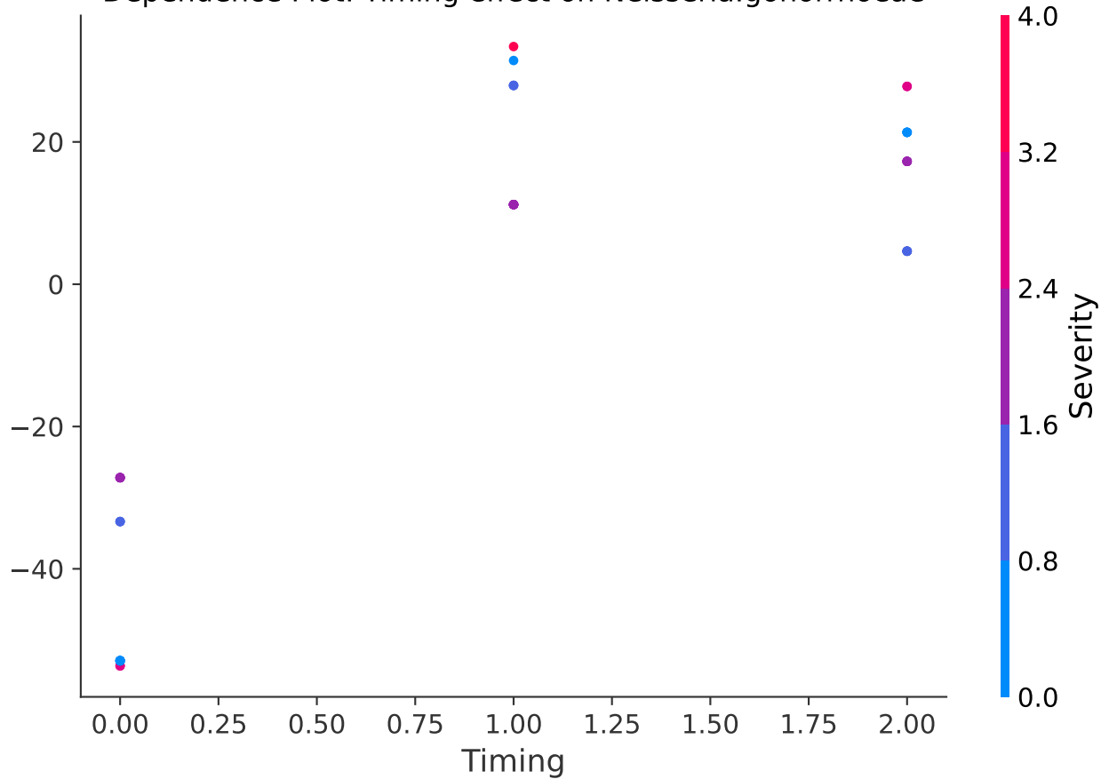
Dependence Plot: Timing effect on Neisseria.gonorrhoeae
