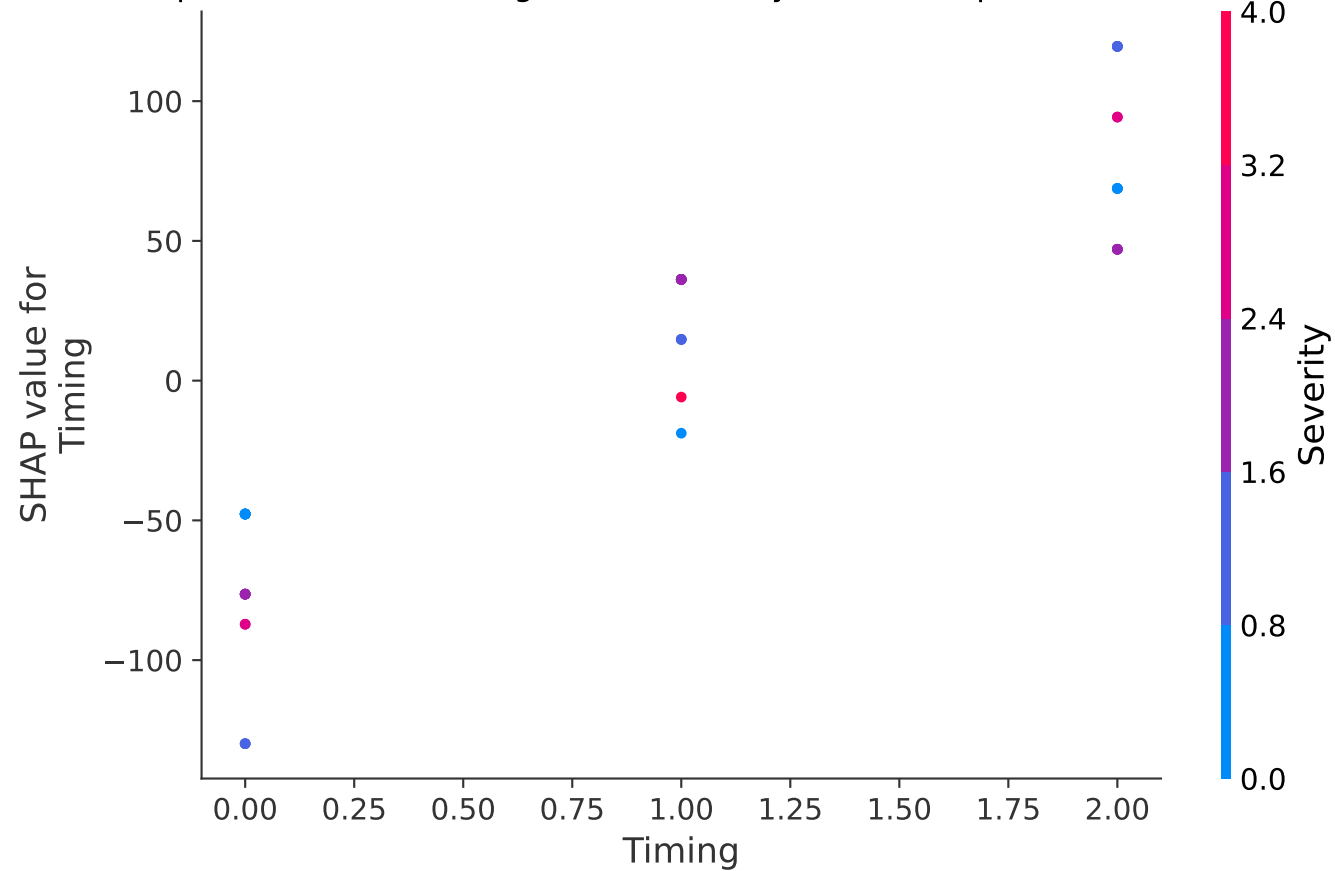
Dependence Plot: Timing effect on Bradyrhizobium.sp.CCBAU.51753
