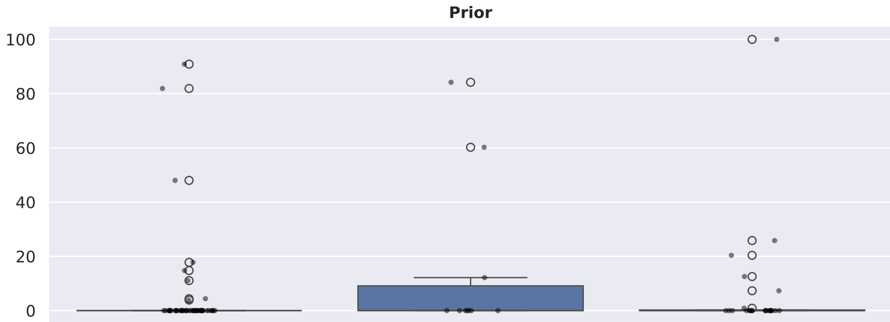
Bacteria: Haemophilus influenzae Abundance by Symptoms Across Time Points
