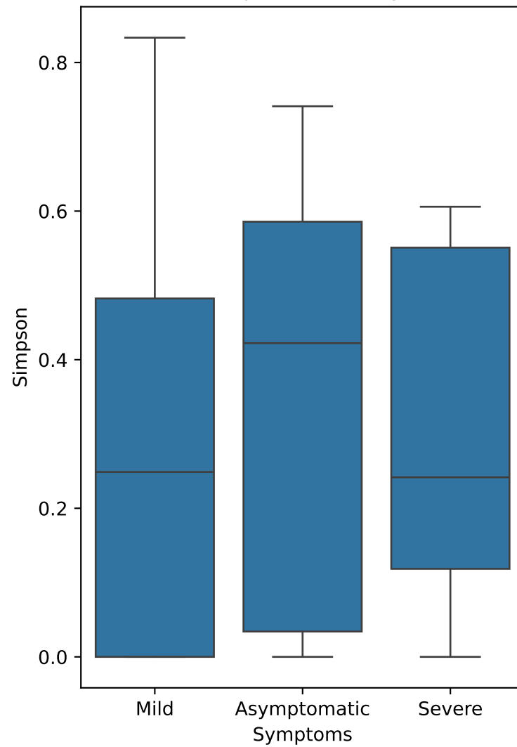
Simpson Diversity
