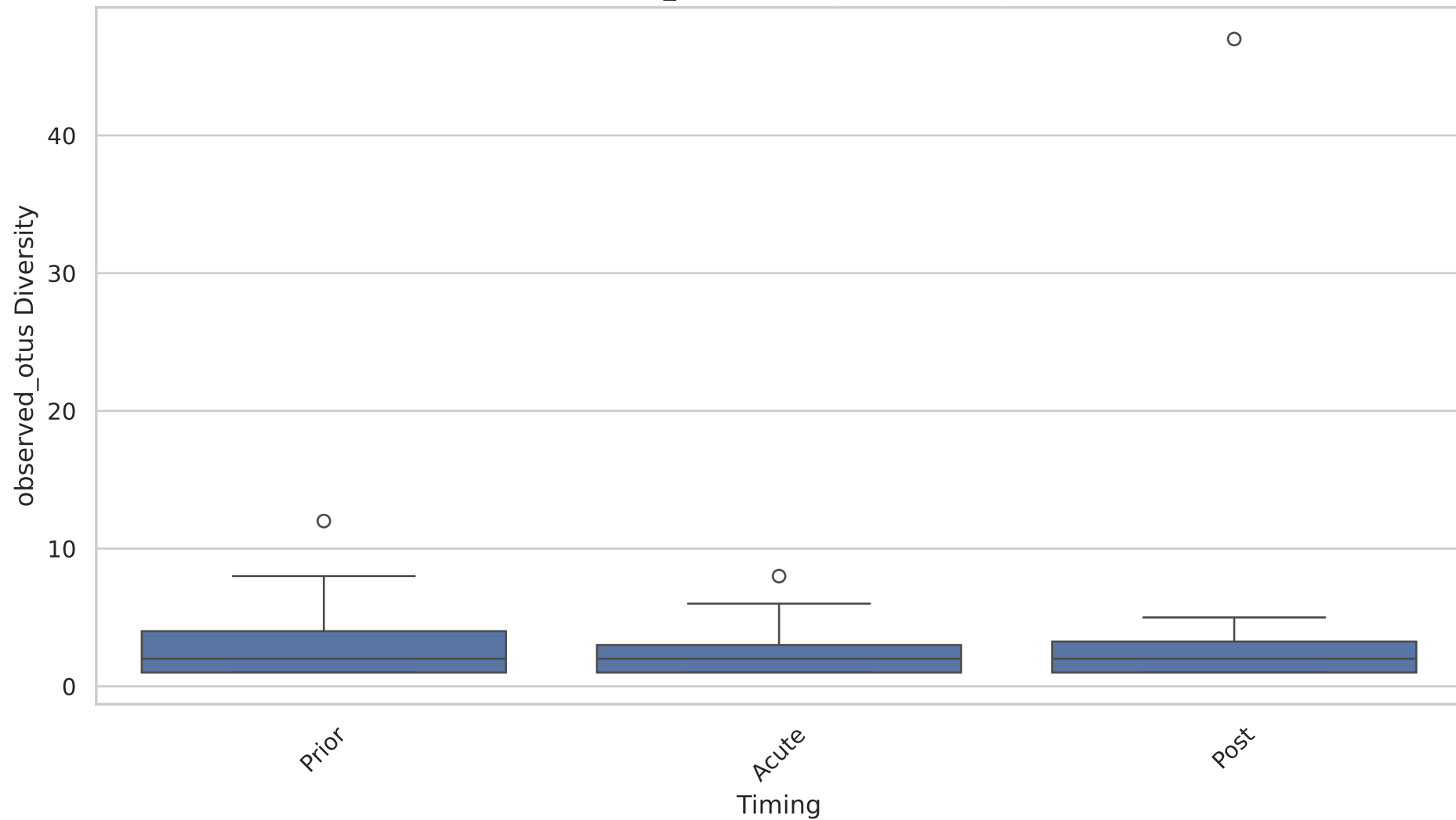
observed_otus Diversity Over Timing
