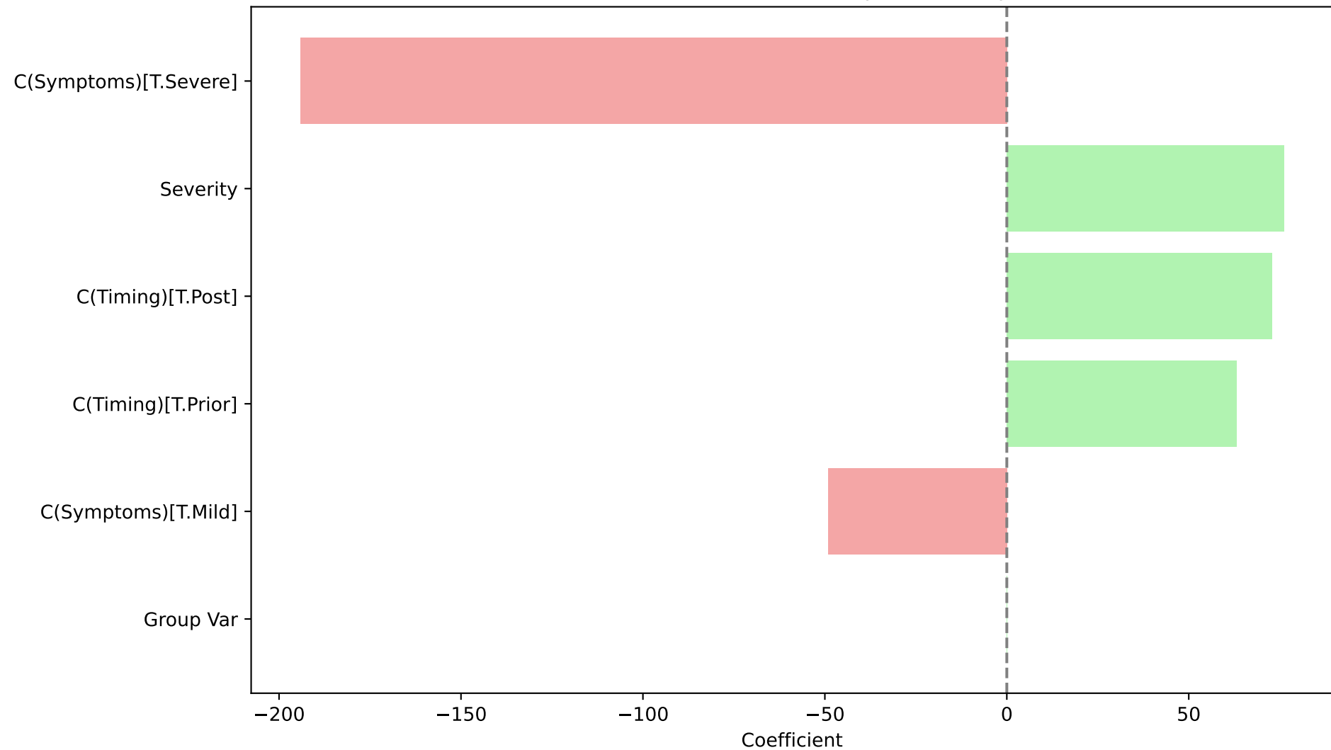
Mixed Model Coefficients: Streptococcus.sp.A12
