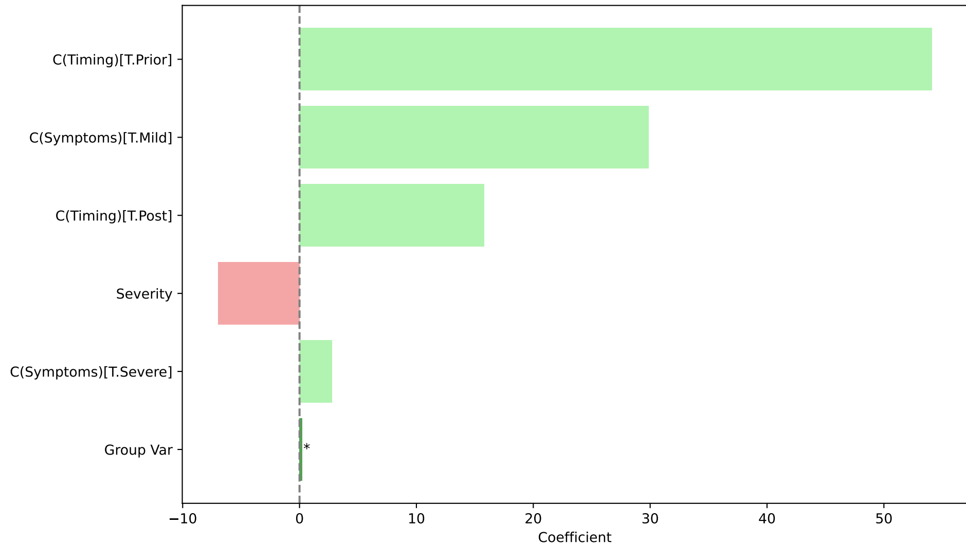
Mixed Model Coefficients: Collinsella.aerofaciens
