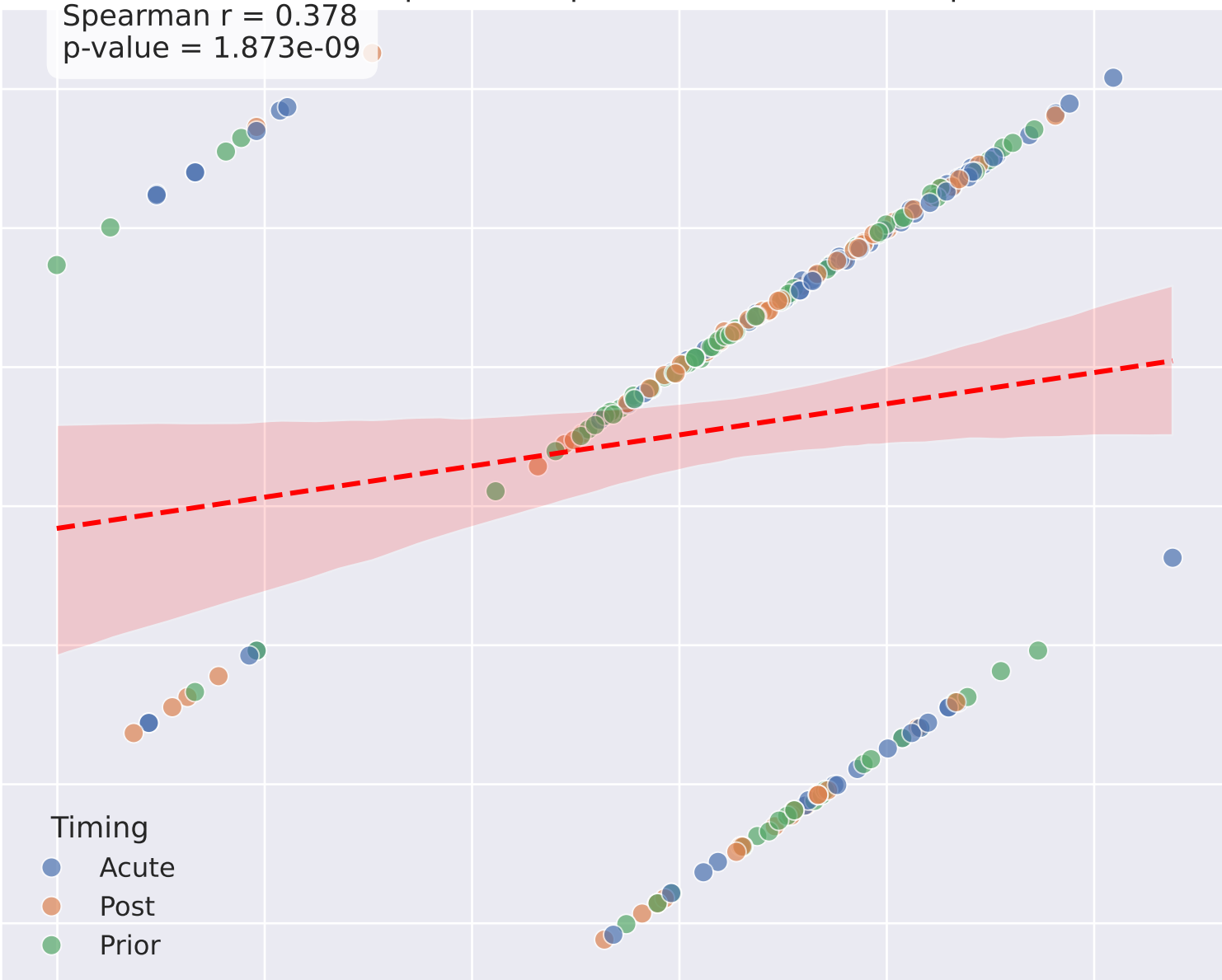
Correlation between Streptococcus.pneumoniae and Haemophilus.influenzae
