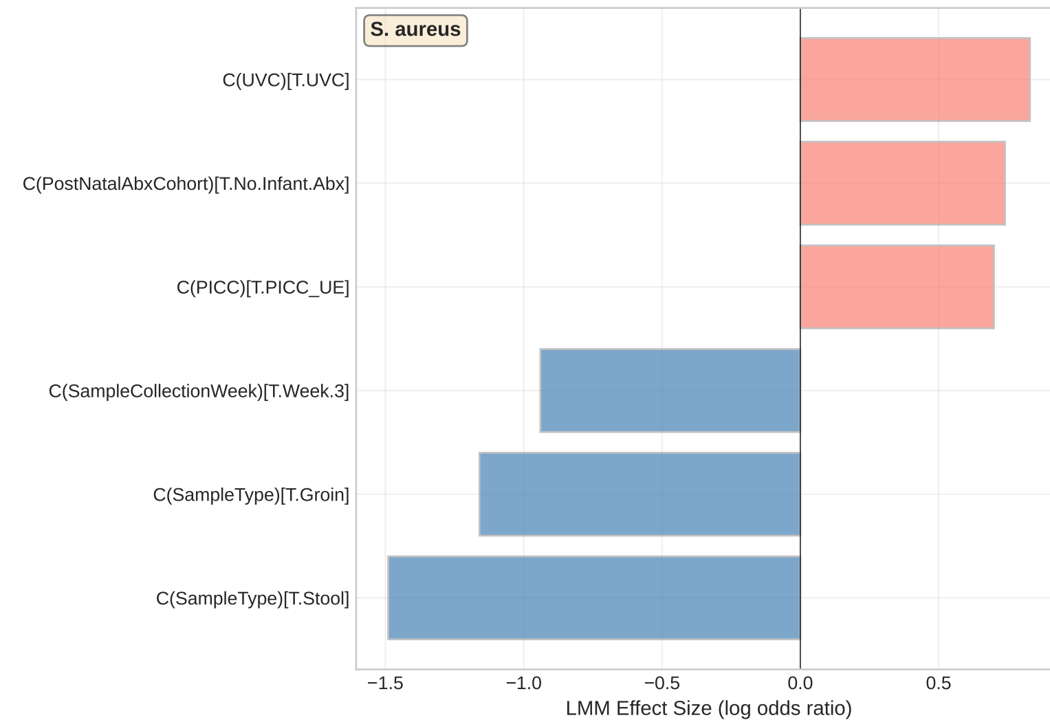
Linear Mixed Model
