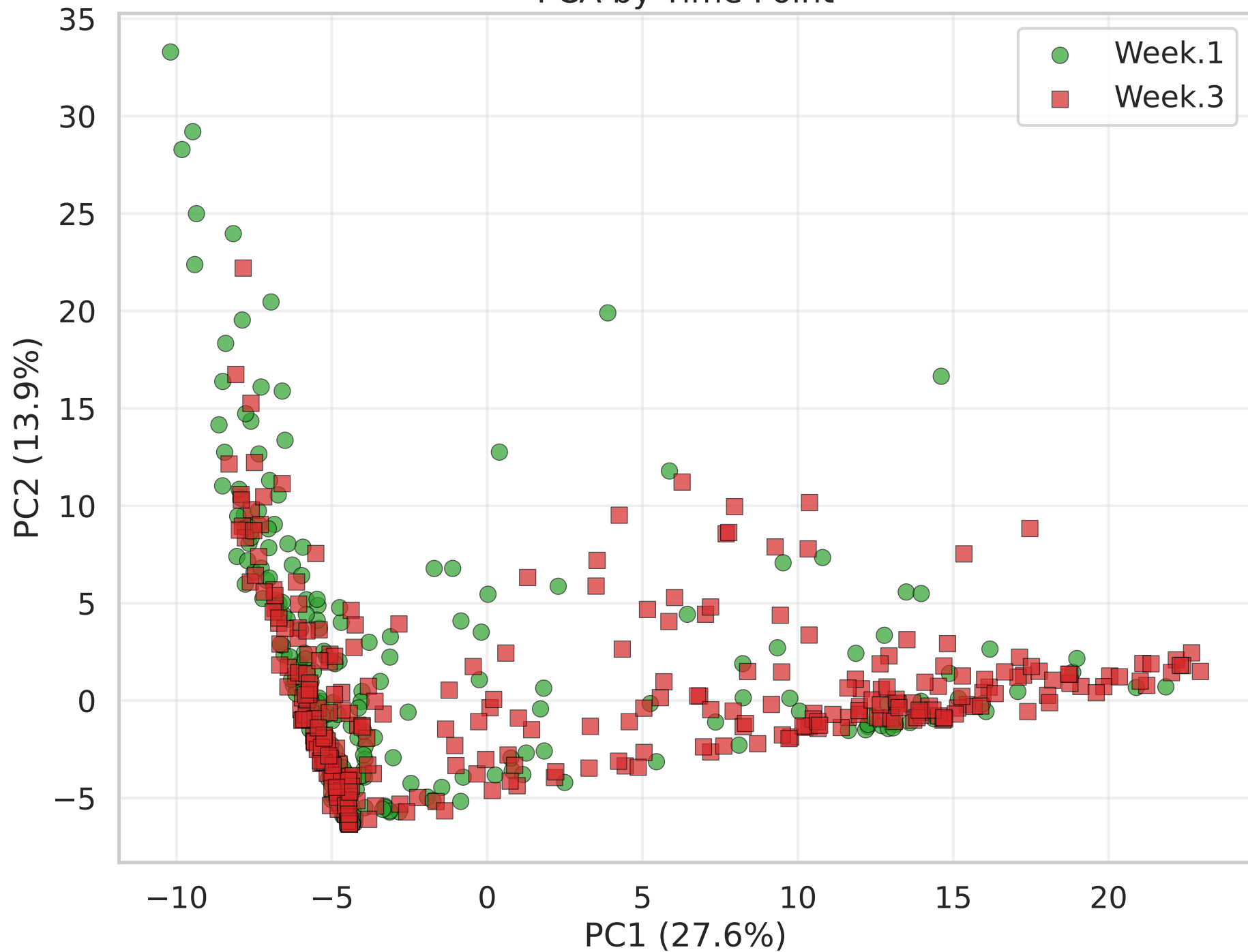
PCA by Time Point
