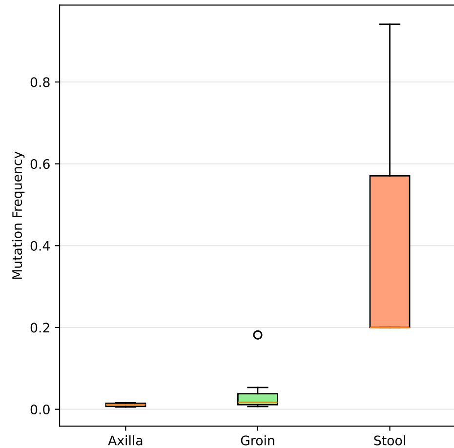
Mycobacterium tuberculosis gyrB 470 G->A (FDR=4.55e-02)
