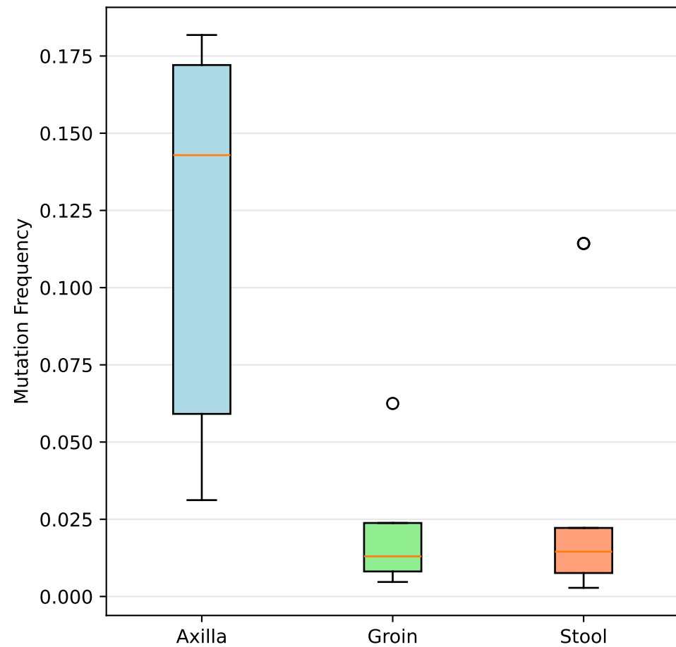
Escherichia coli gyrA 83 S->A (FDR=4.55e-02)
