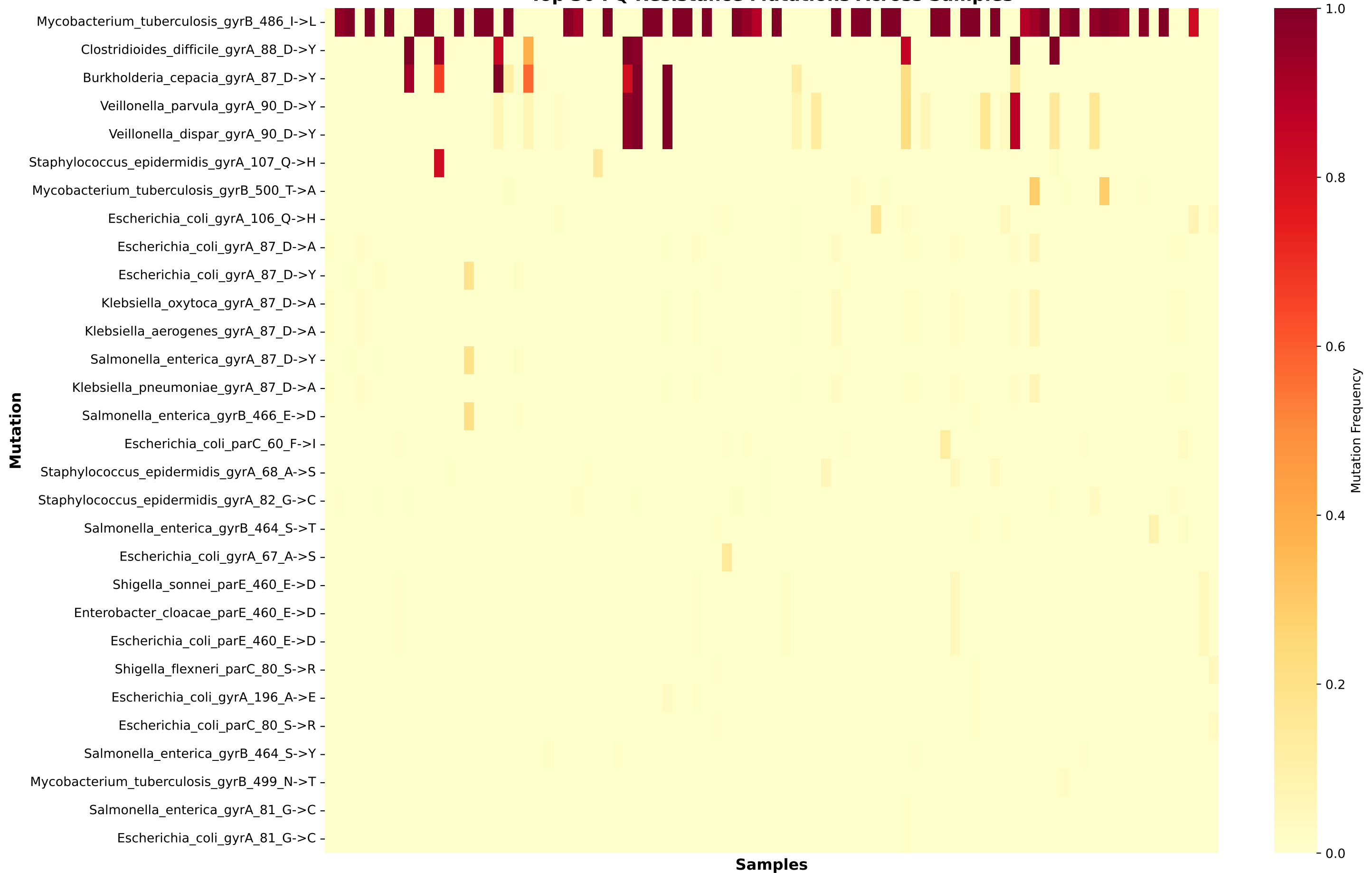
Top 30 FQ Resistance Mutations Across Samples
