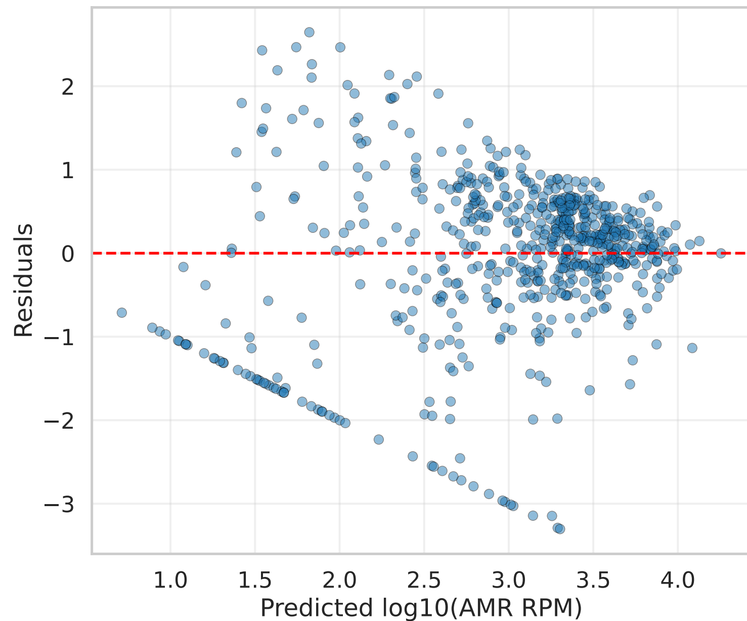
Residual Plot
