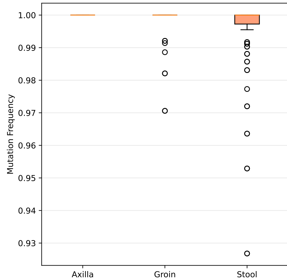
Enterococcus faecalis gyrA 87.0 E/S->K (FDR=2.85e-03)
