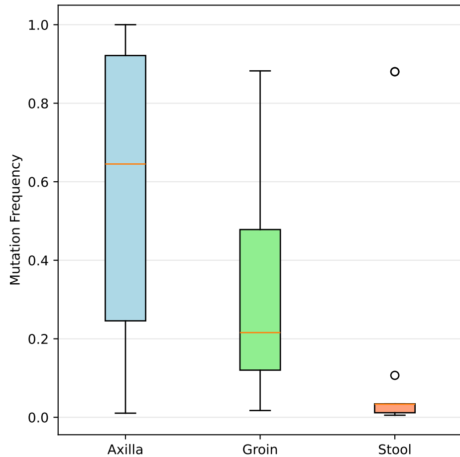
Staphylococcus aureus parE 432.0 D/S->V (FDR=6.32e-07)
