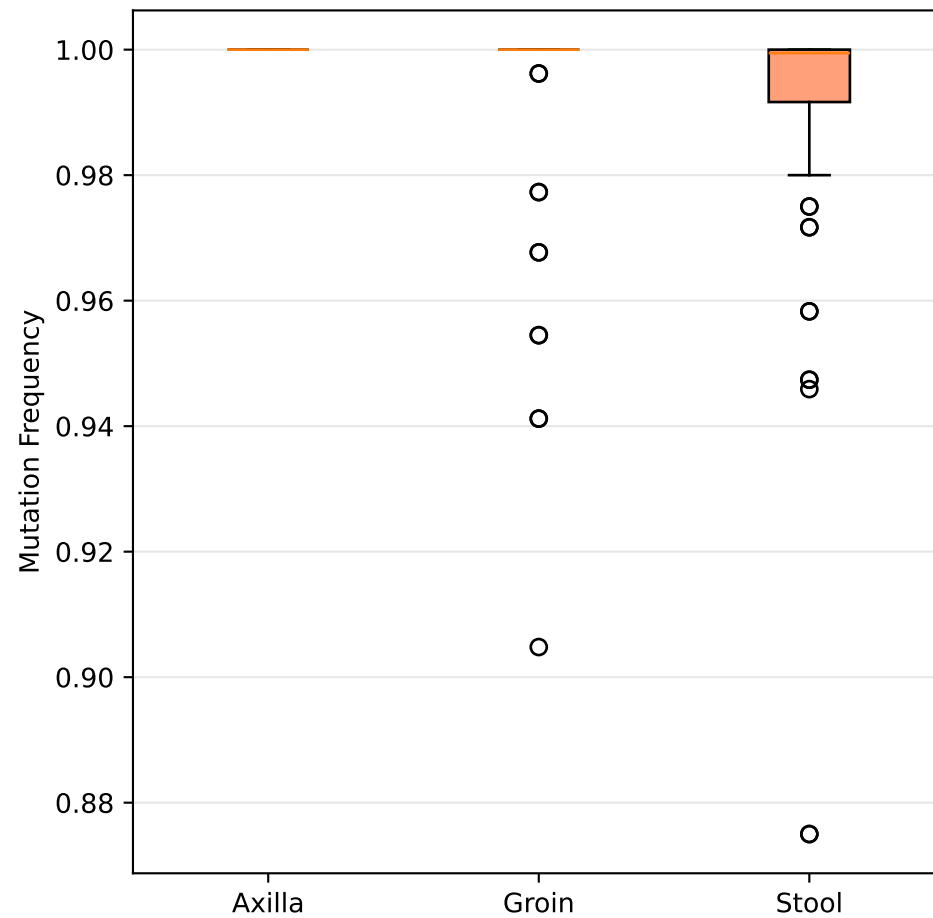
Klebsiella pneumoniae gyrA 154.0 K->R (FDR=1.24e-05)
