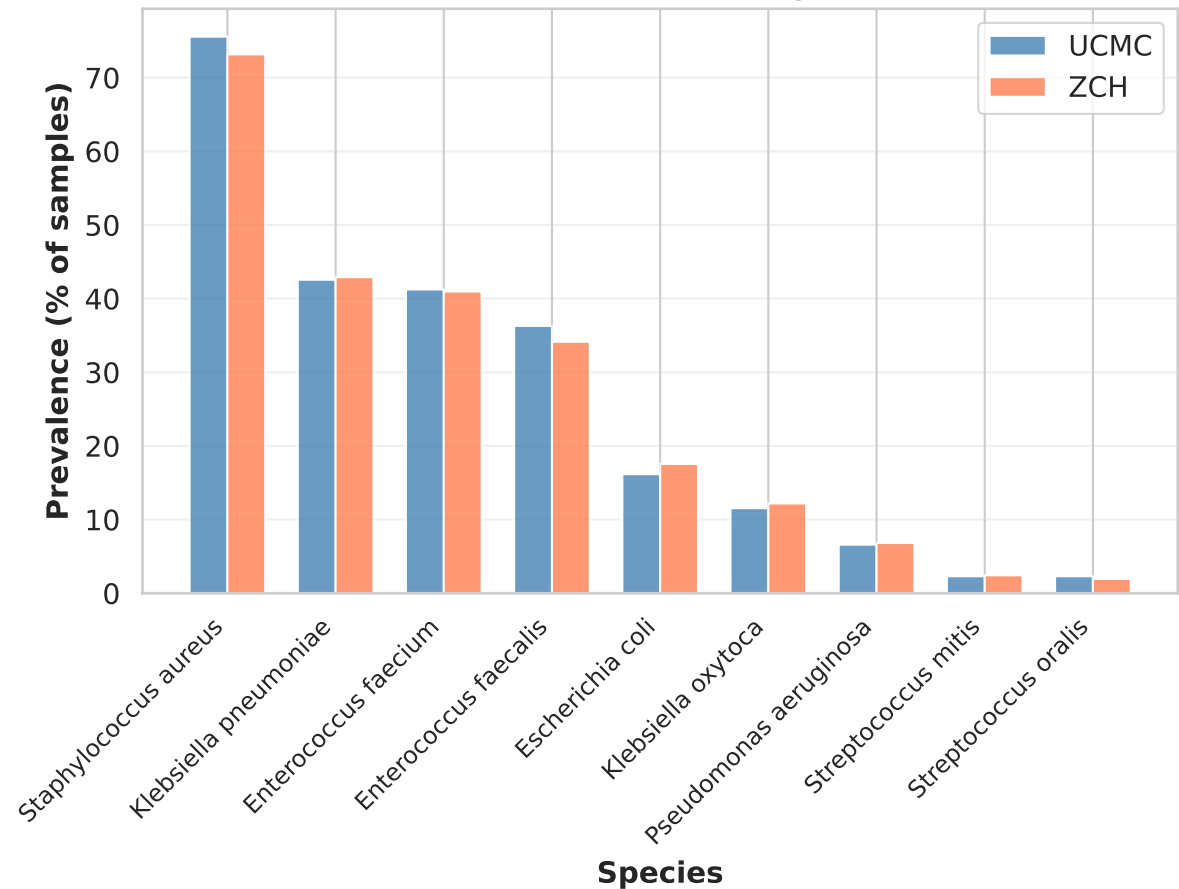
B. Species Prevalence by Location
