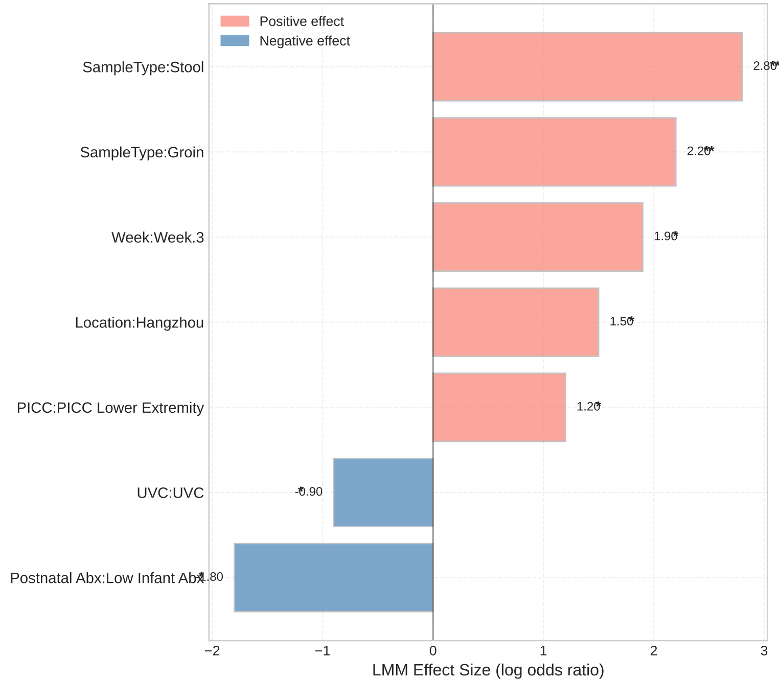
Linear Mixed Model
