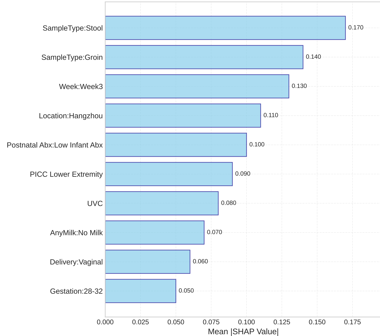
Random Forest (SHAP Importance)
