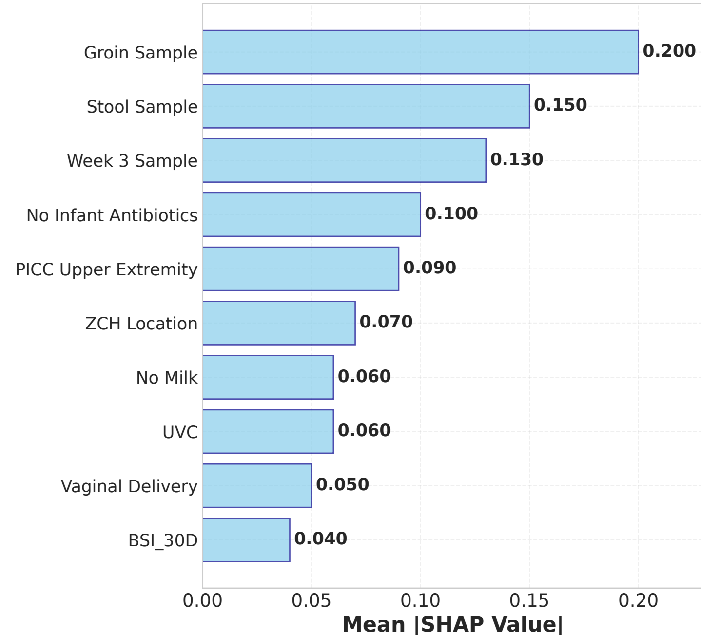
Random Forest (SHAP Importance)
