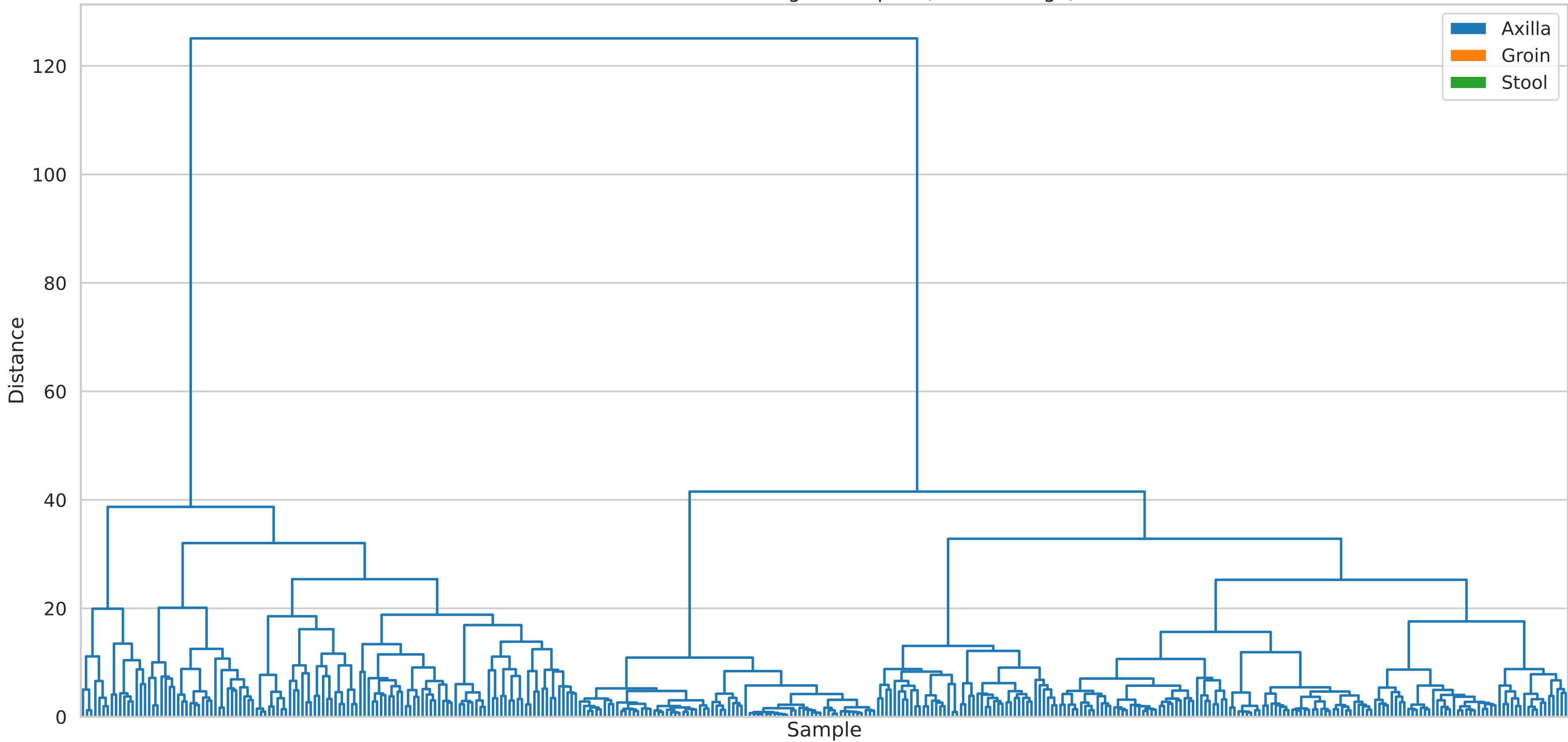
Hierarchical Clustering of Samples (Ward Linkage)
