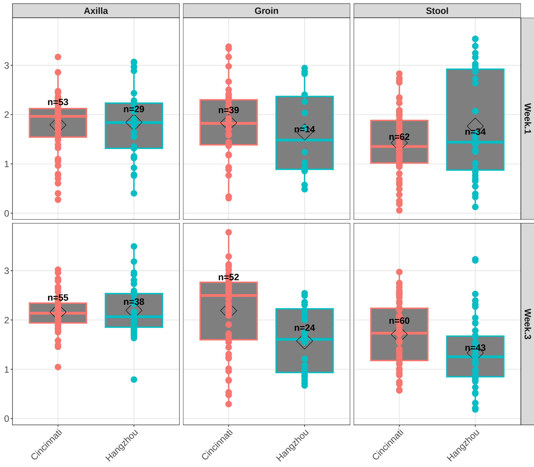
Shannon Diversity Index
