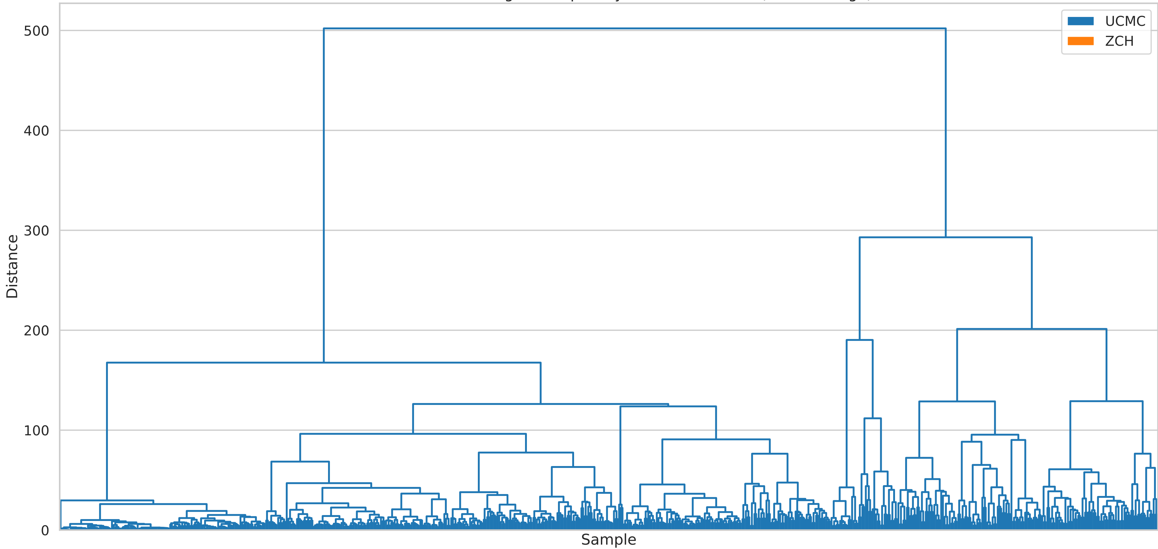
Hierarchical Clustering of Samples by AMR Gene Profile (Ward Linkage)
