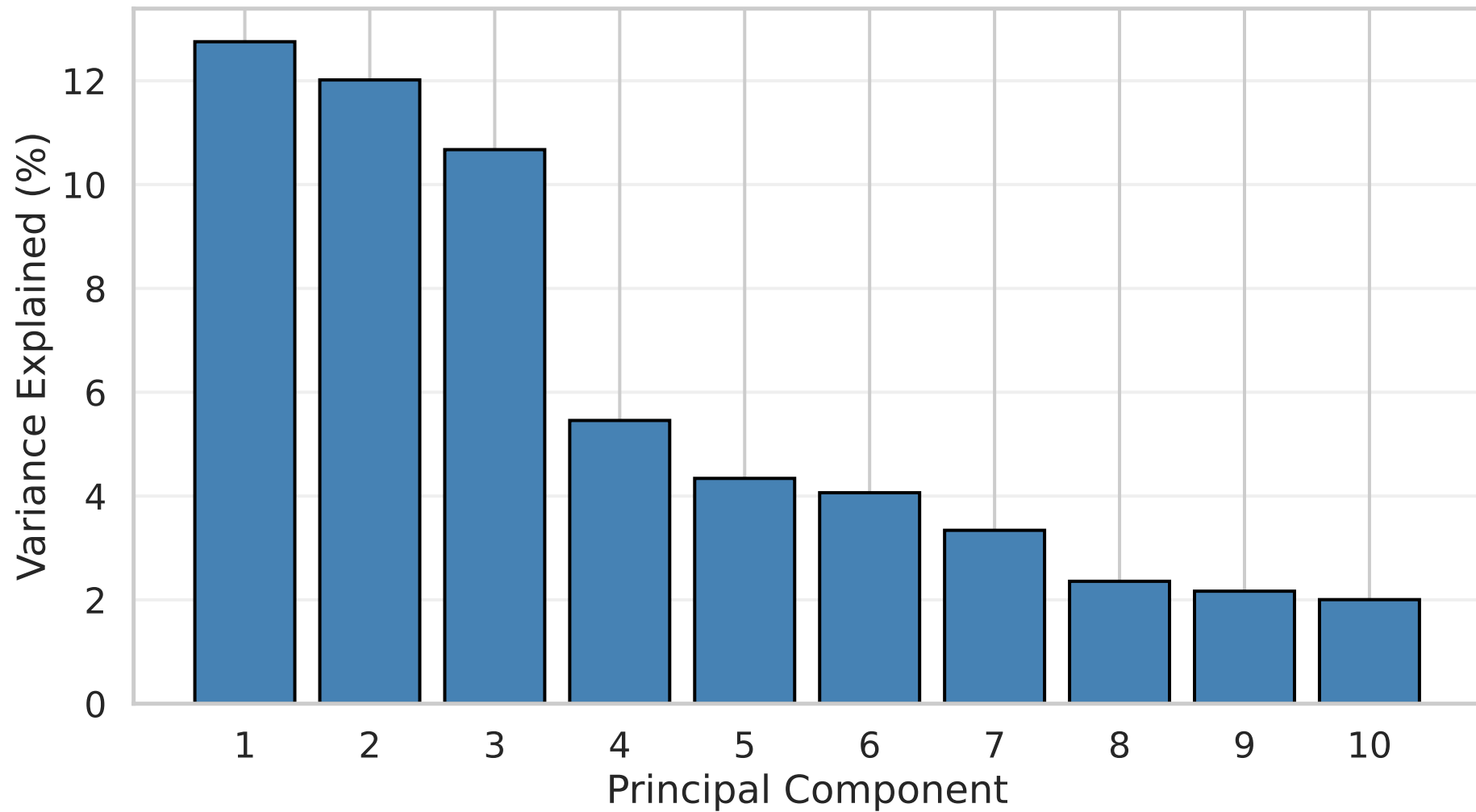
PCA Scree Plot
