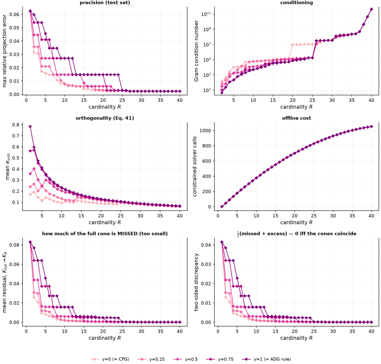
Figure 11: The whole family on 3D Pellet-Cladding. Precision and the two cone-residual panels show a clean monotone fan in \gamma : every member reaches the same floor, higher \gamma simply reaches it later ( R \approx 15 at \gamma = 0 against R \approx 25 at \gamma = 1 ), so the cost of the weight is a delay rather than a worse asymptote. The offline-cost panel has all five curves exactly superimposed — this is the panel that shows the knob is free. Conditioning is the one panel where the ordering is not monotone throughout: it inverts near R \approx 20 , discussed below.
