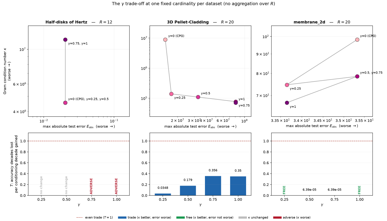
Figure 12: Top: \kappa against absolute test error, one point per \gamma , at the fixed R named in each title. Coincident members share one label. Bottom: the exchange rate (11) where it is defined, and the regime otherwise. Half-disks is the null case: \gamma \leq 0.5 selects the same cone as CPG and \gamma \geq 0.75 is strictly adverse. Pellet-Cladding shows a sharp corner at \gamma = 0.25 . Membrane shows no trade at all — every member is free or neutral.
