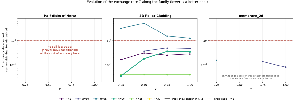
Figure 13: The exchange rate (11) against \gamma , one curve per cardinality; the curve at the R used in §7.2 is drawn thick. \gamma = 0 is absent by construction — it is CPG against itself, so both logarithms vanish — and a point is plotted only where T is a meaningful number, so gaps are cells that were free, \kappa -neutral or adverse rather than missing runs. Half-disks has no trade at any cardinality below its rank cliff. On Pellet-Cladding the R = 15 curve sits above the even-trade line for every \gamma while R = 25 sits an order of magnitude below it, so the same knob is poor value at one cardinality and excellent at another. Membrane has so few trades that three points are all the family produces at these R .
