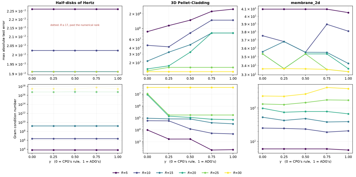
Absolute test error and conditioning as functions of \gamma — one curve per cardinality
