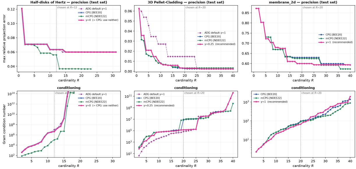
Each dataset's recommended \gamma against CPG and mCPG (the recommendation differs per dataset)
