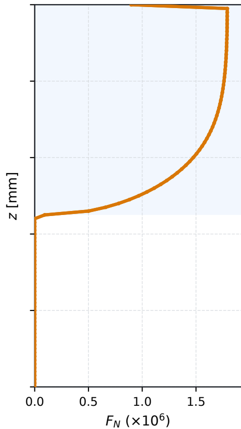
Contact normal-force profile, u_z = 0.210 mm (snapshot 6)
