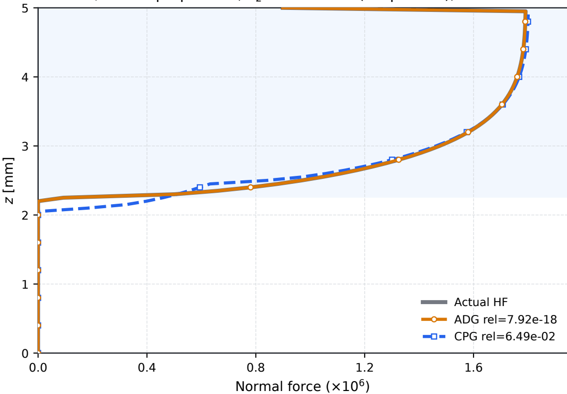
HF/ROM superposition, u_z = 0.210 mm (snapshot 6), best ADG
