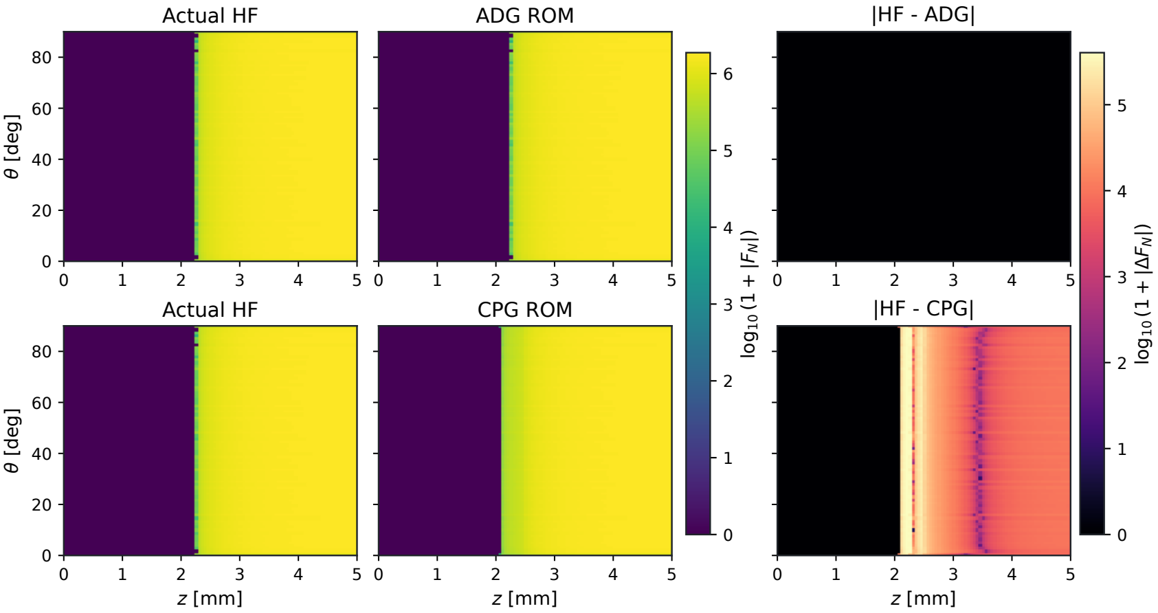
Unwrapped quarter-cylinder contact surface, u_z = 0.210 mm (snapshot 6)
