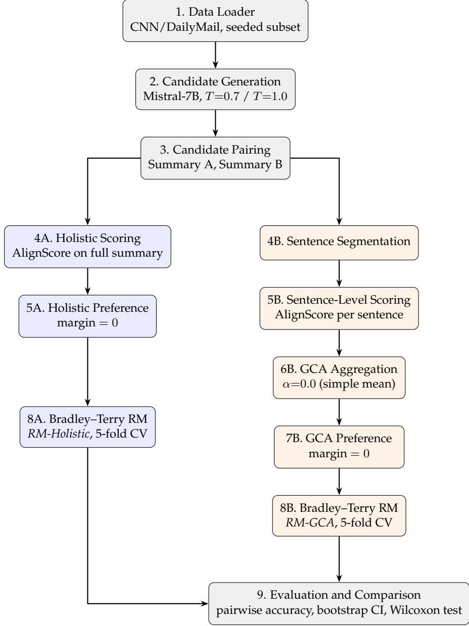
Figure 4.1.: The final pipeline. Shared setup (grey) produces one candidate pool from which two independent preference-construction branches run: holistic (blue) and GCA (orange). Each branch trains its own Bradley-Terry reward model under an identical recipe, and the two are compared in the final evaluation step. Compare to the pipeline described in the original proposal (Section 4.9), which additionally included a DPO fine-tuning stage and a cross-summary sentence-alignment step, neither of which appears here. Chapter 5, Section 5.1 walks through every stage’s concrete input and output.
