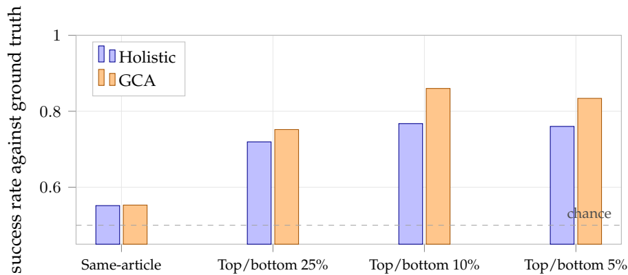
Figure 6.6.: Ground-truth precision at n = 1,000 (Table 6.14). GCA is indistinguishable from holistic on the closest comparison and ahead on all three constructions with a genuine quality gap, significantly so on two of the three.
