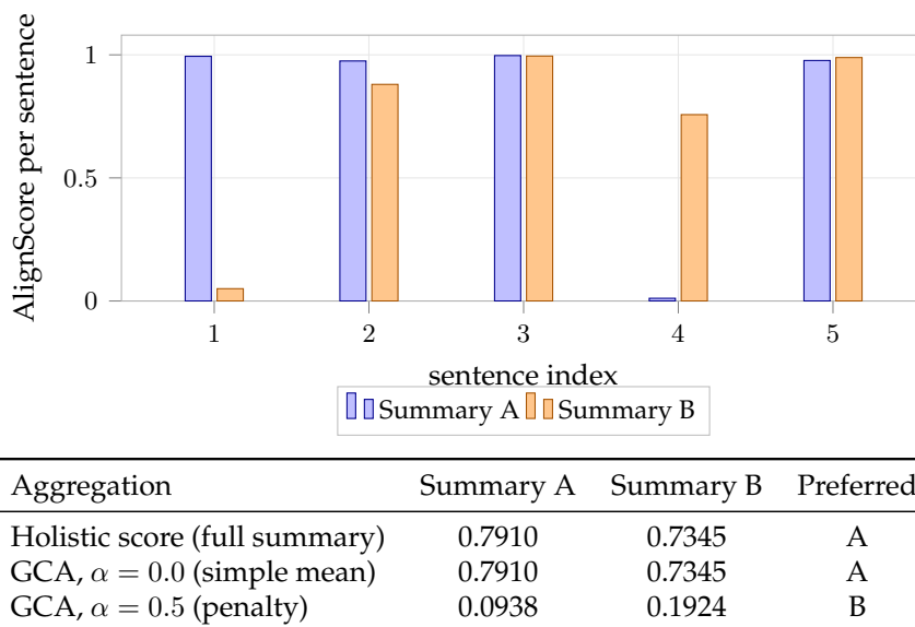
Figure 3.1: Worked example on pair cnn_00233 from the n = 200 preference set (evaluator mode nli_sp ). Summary A has one sentence scored 0.011 among four strong ones. The simple mean preserves the holistic ordering, while the \alpha = 0.5 penalty inverts it. Values are computed from the stored per-sentence scores in data/preferences/gca_reward_preferences_200.jsonl .
