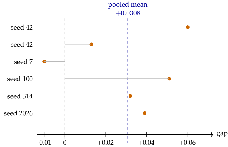
Figure 6.3: Per-run GCA–Holistic accuracy gap at n = 1,000 , against the pooled mean. Five of six runs favor GCA, but the spread across runs is wide relative to the pooled effect, which is why no single run was treated as conclusive.
