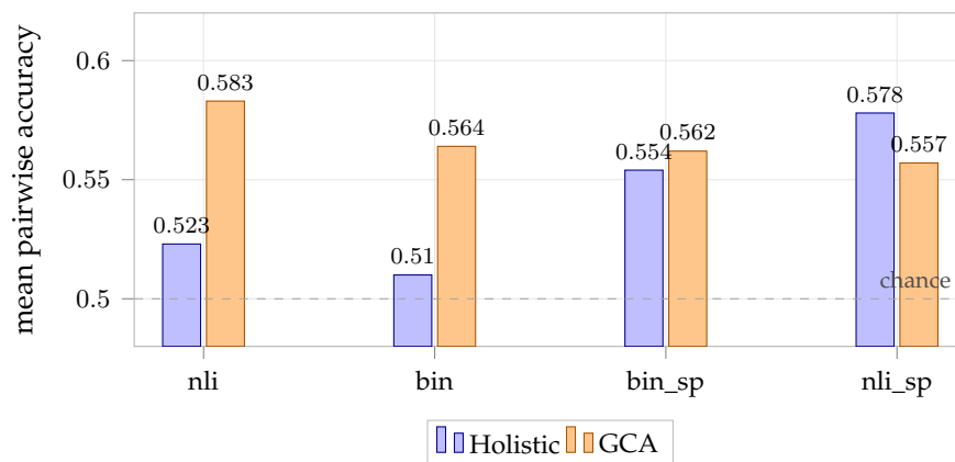
Figure 6.2: Evaluator-mode sweep ( n = 1,000 , \alpha = 0.0 ). The two left-hand modes do not split the input internally; the two right-hand modes do. Each bar is a single run, so differences of this size fall within the run-to-run variation documented in Section 6.6, and the comparison is exploratory.
