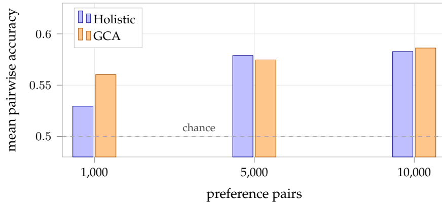
Figure 6.4: Accuracy at the three dataset sizes. Absolute accuracy rises for both conditions as data is added, while the difference between them contracts. Only the n = 1,000 bars are averaged over repeated runs; the other two are single runs on datasets that are nested supersets of the n = 1,000 set (Chapter 4, Section 4.6).
