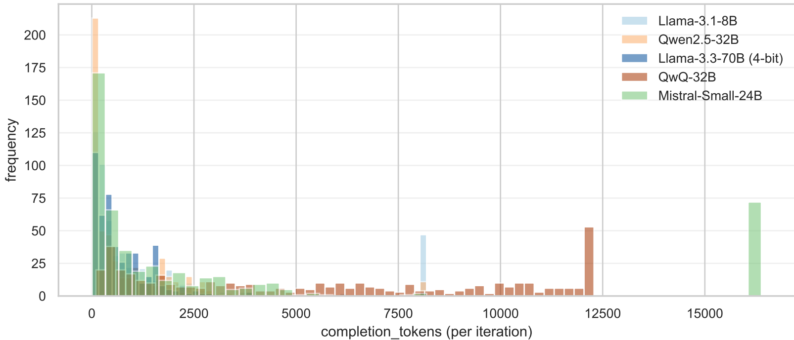
Plot 11 — Per-iteration completion-token distribution by model
