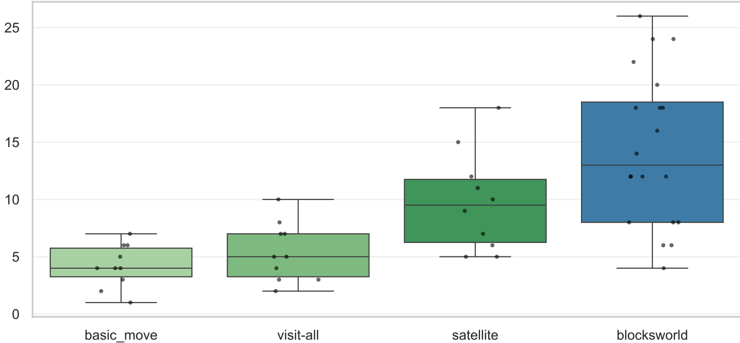
Plot 12 - Reference plan length per domain (ground-truth difficulty)
